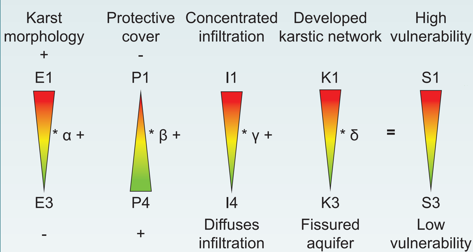
Fig 2 : EPIK method
