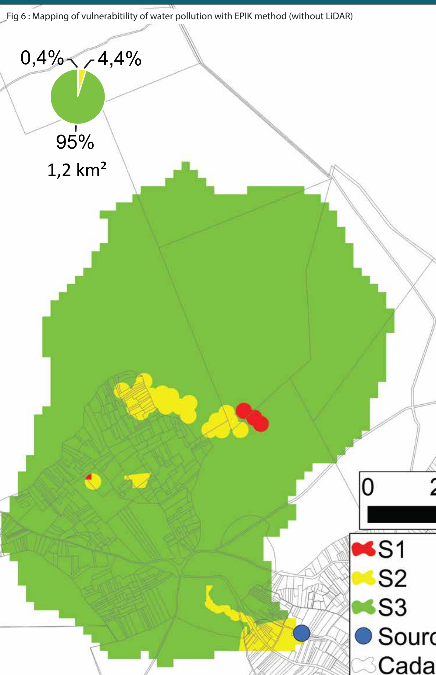
Fig 6 : Mapping of vulnerability of water pollution with EPIK method (without LiDAR)
