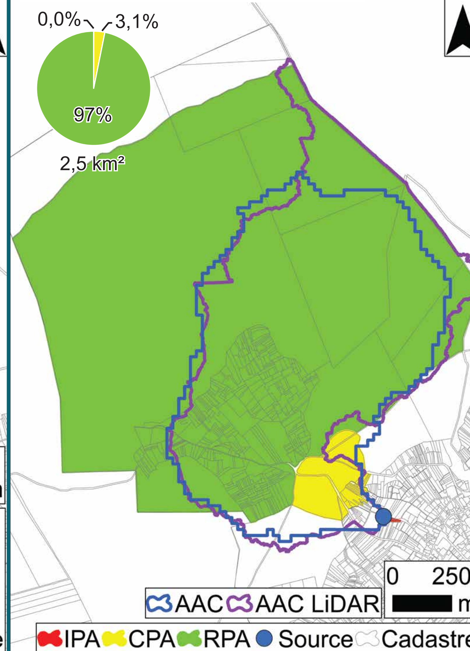
Fig 8 : Comparison between the PPC of the Trépail drinking water source and the vulnerability maps
