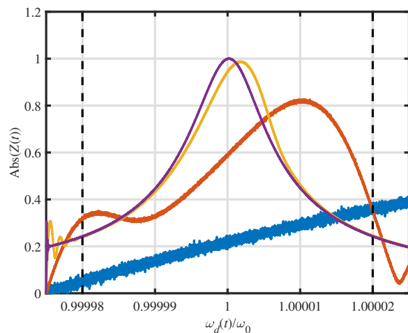
Fig. 3. Simulated amplitude of resonator response, for T_{sweep} = [1, 10, 10^2, 10^3] \times Q/\omega_0 (resp. blue, orange, yellow, purple lines) in the presence of measurement noise (the same amount as for deriving the results of Fig. 2).
