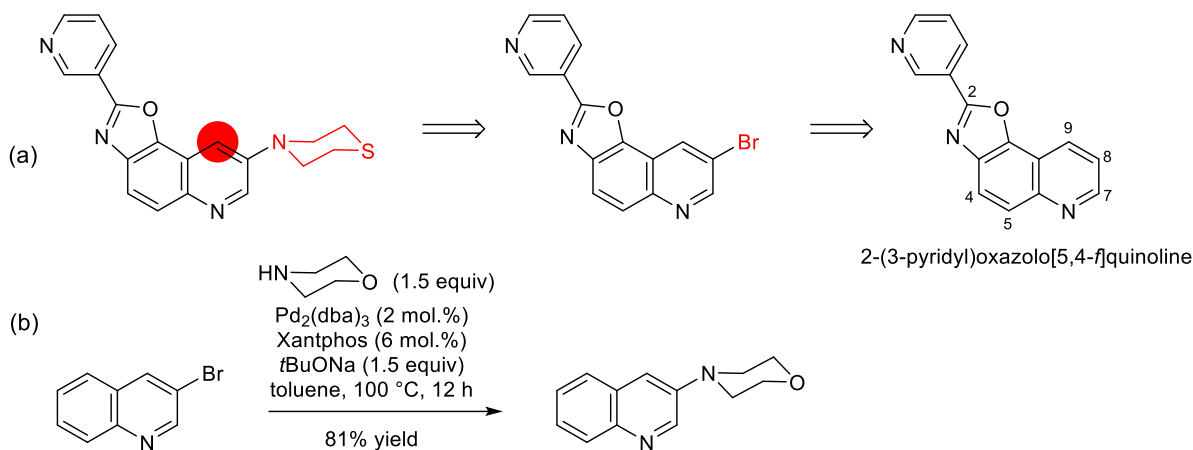
Scheme 4. (a) Retrosynthesis plan to access the quinoline analog of CD-07 and (b) preliminary results.
