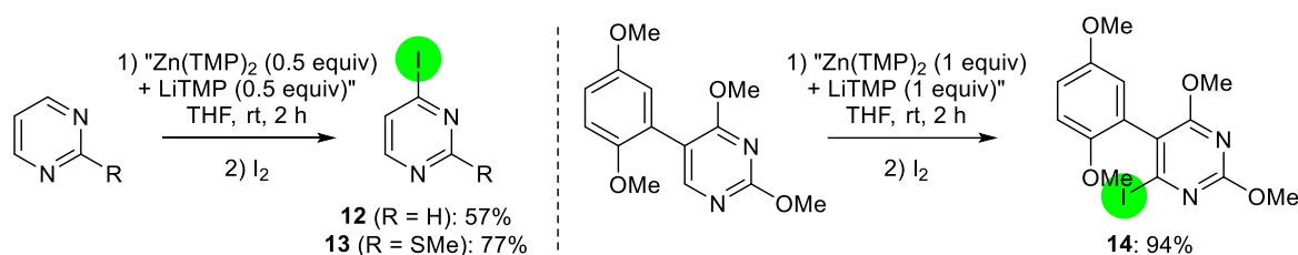
Scheme 11. Functionalization of pyrimidine, 2-(methylthio)pyrimidine ( left ) and 2,4-dimethoxy-5-(2,5-dimethoxyphenyl)pyrimidine ( right ) toward the iodides 12 – 14 , respectively, by deprotonation with in situ trapping followed by iodolysis.
