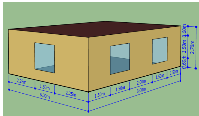
Figure 7: Test building.
