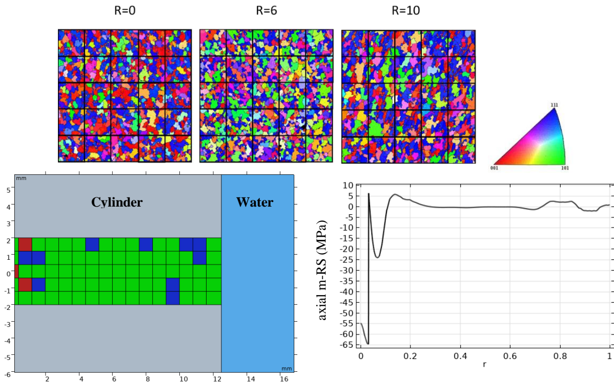
Figure 4. a) 5 \times 5 grid over the real microstructure of the material investigated b) distribution of the high yield stress grains along sample radial direction, inverse pole figure, IPF, coloring reference for the extrusion axis and b) axial intergranular stress profile along radial direction.
