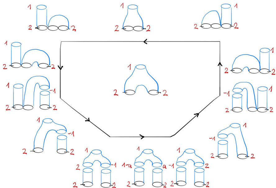
FIGURE 9. The hexagon of Floer annuli
