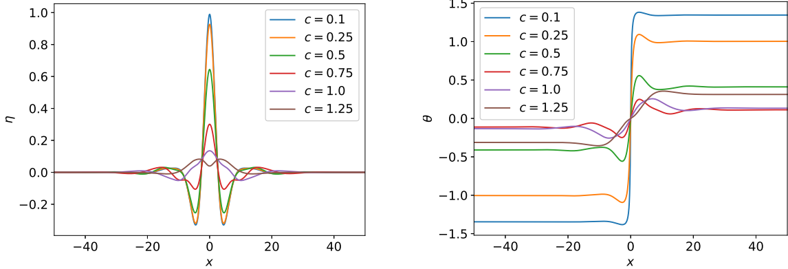
FIGURE 18. Numerically computed solitons for potential (E2) with \lambda = 3.0 , showing \eta_k (left panel) and \theta_k (right panel) as function of x_k .
