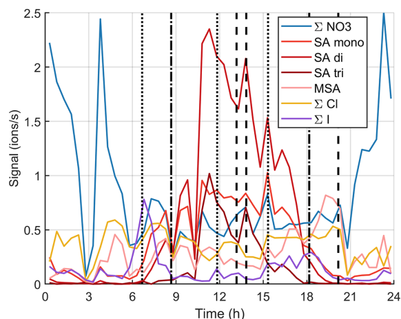
Figure B8. Simplified version of variation of signals of different anions during one marine growth event on 15 October 2020. The dotted vertical lines show the start times of the growth events and the dashed lines show their end times.
