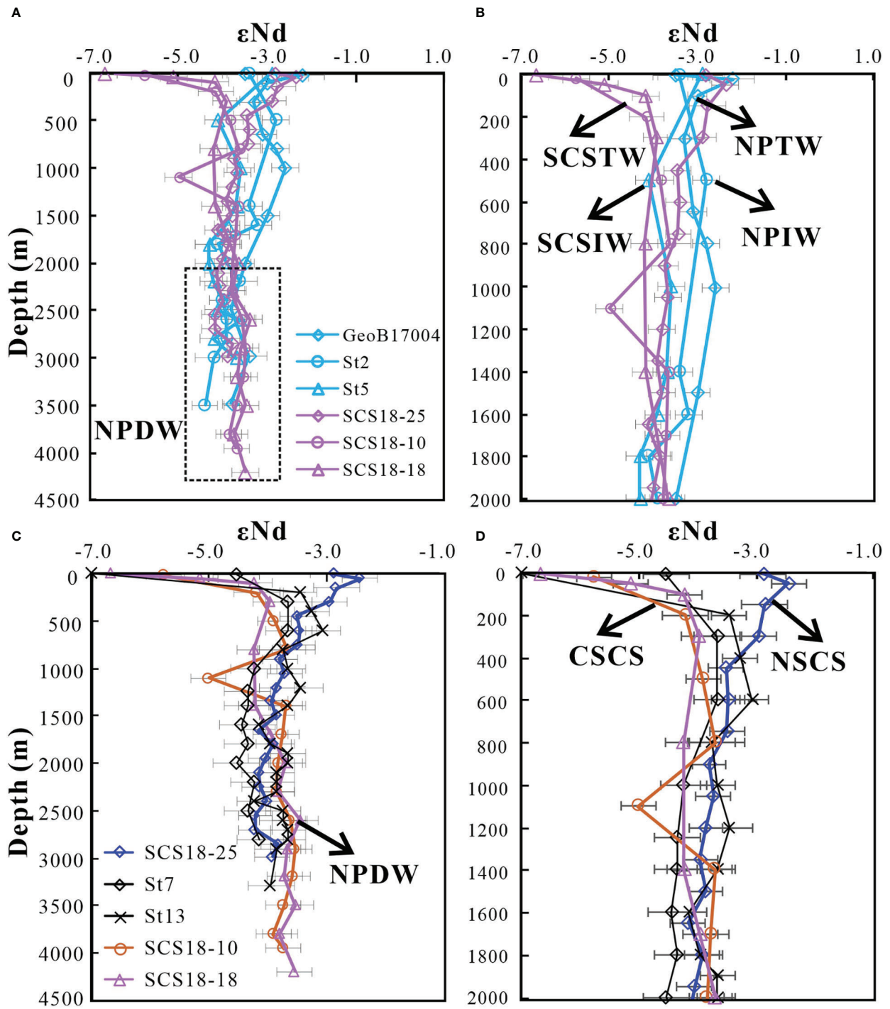
FIGURE 9 Comparisons of \epsilon\text{Nd} vertical profiles between the SCS and the North Pacific (A, B), and within the SCS (C, D). \epsilon\text{Nd} values of the North Pacific are from Wu et al. (2015); Behrens et al. (2018b).
