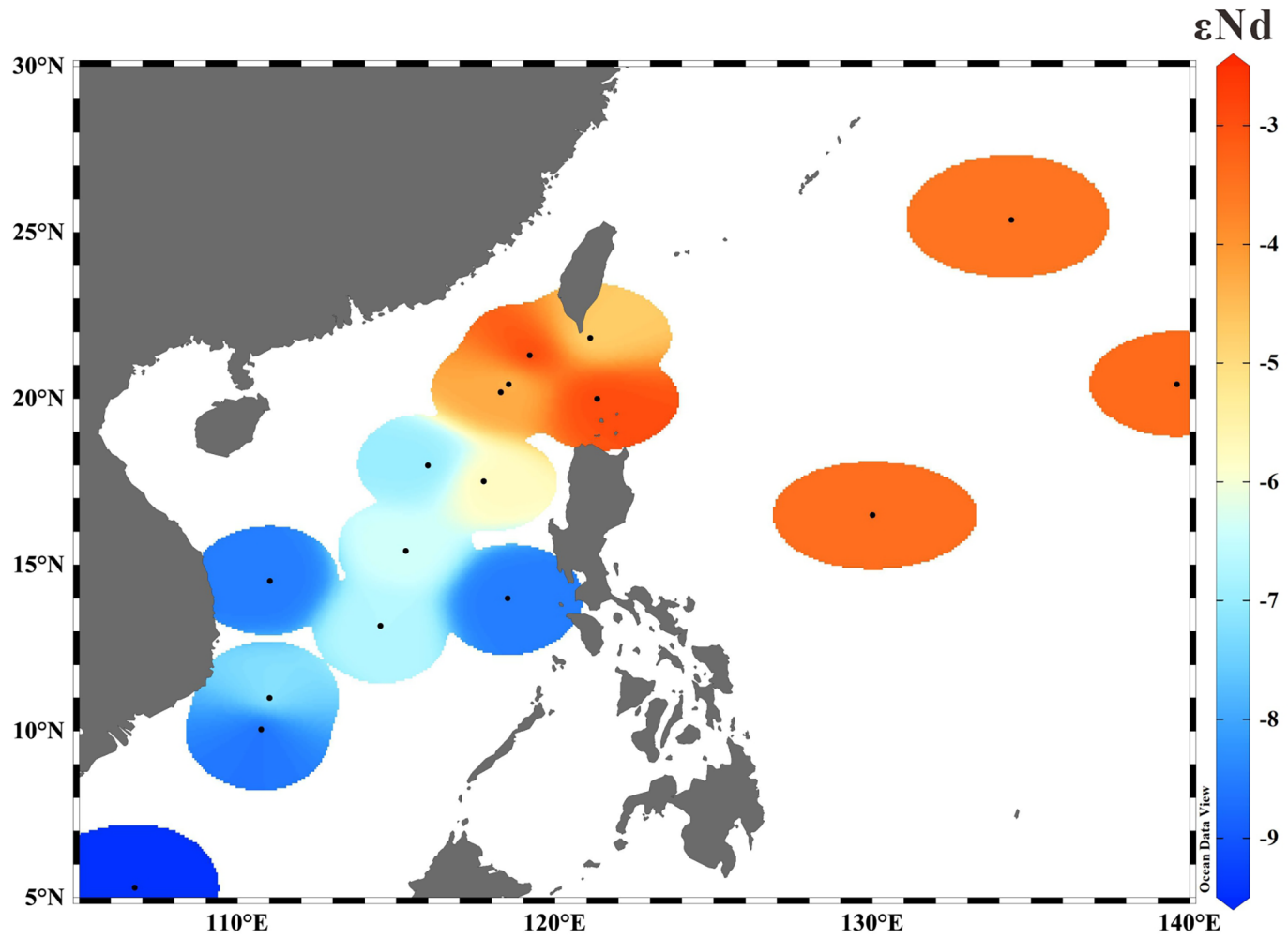
FIGURE 7 Distribution of surface water \epsilon Nd in the SCS and West Pacific. Data sources: this study, Amakawa et al. (2000), Wu et al. (2015), and Behrens et al. (2018b). The figure was created using Ocean Data View (Schlitzer, 2014).
