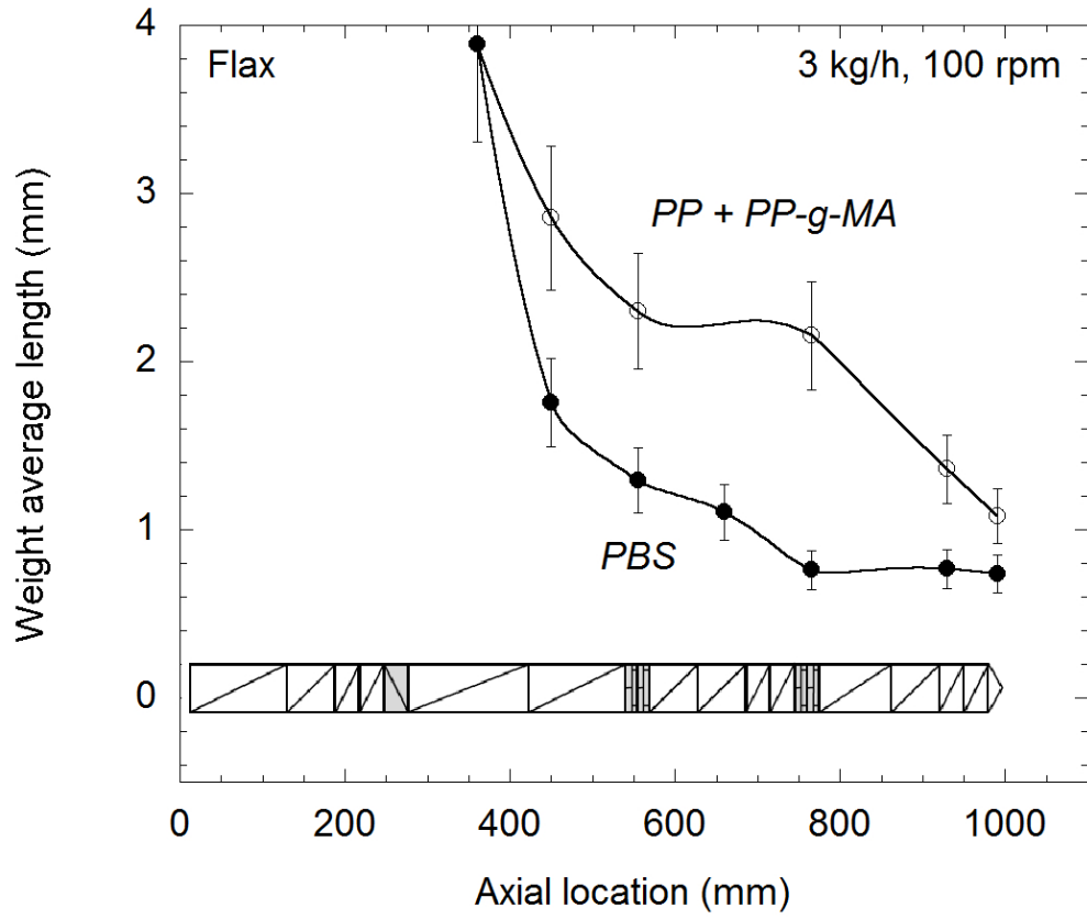
Figure 3. Changes in weight average fiber length along the screws for a fixed processing condition. Lines are just to guide the eyes.
