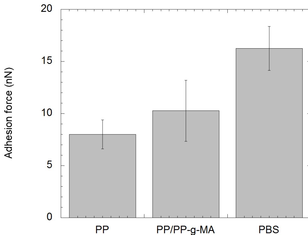
Figure 14. Intermolecular adhesion forces between nanocrystalline cellulose functionalized AFM levers with PP, PP/PP-g-MA and PBS at 25°C and 45% RH.
