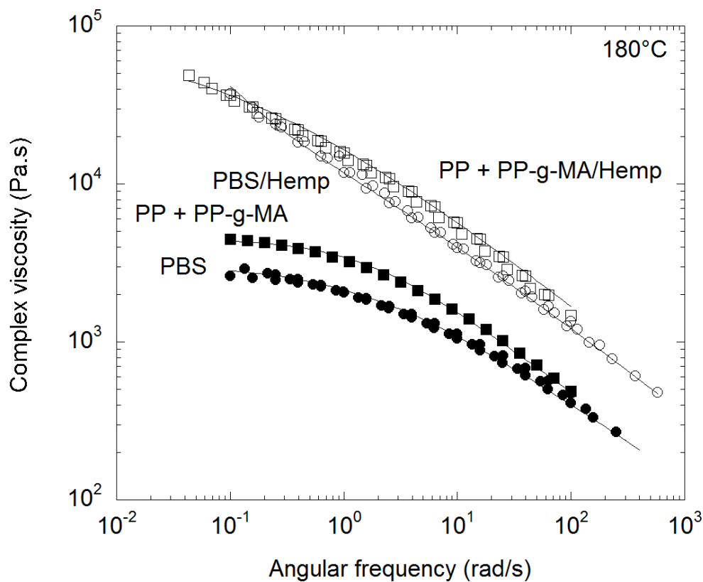
Figure 9. Complex viscosity curves of the two matrices and the corresponding hemp-based composites at 180°C. Full lines are fits with a Carreau-Yasuda model.
