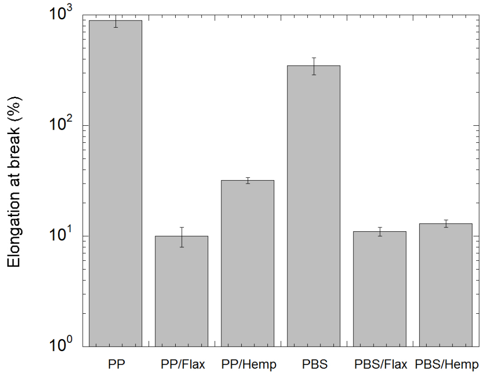
Figure 11. Mechanical properties of the various composites. (a) Relative Young's modulus, (b) Stress at break, (c) Elongation at break. PP means PP/PP-g-MA.
