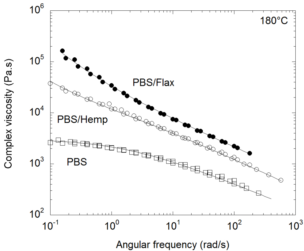
Figure 8. Complex viscosity curves of PBS and PBS-based composites at 180°C. Full lines are fits with a Carreau-Yasuda model.
