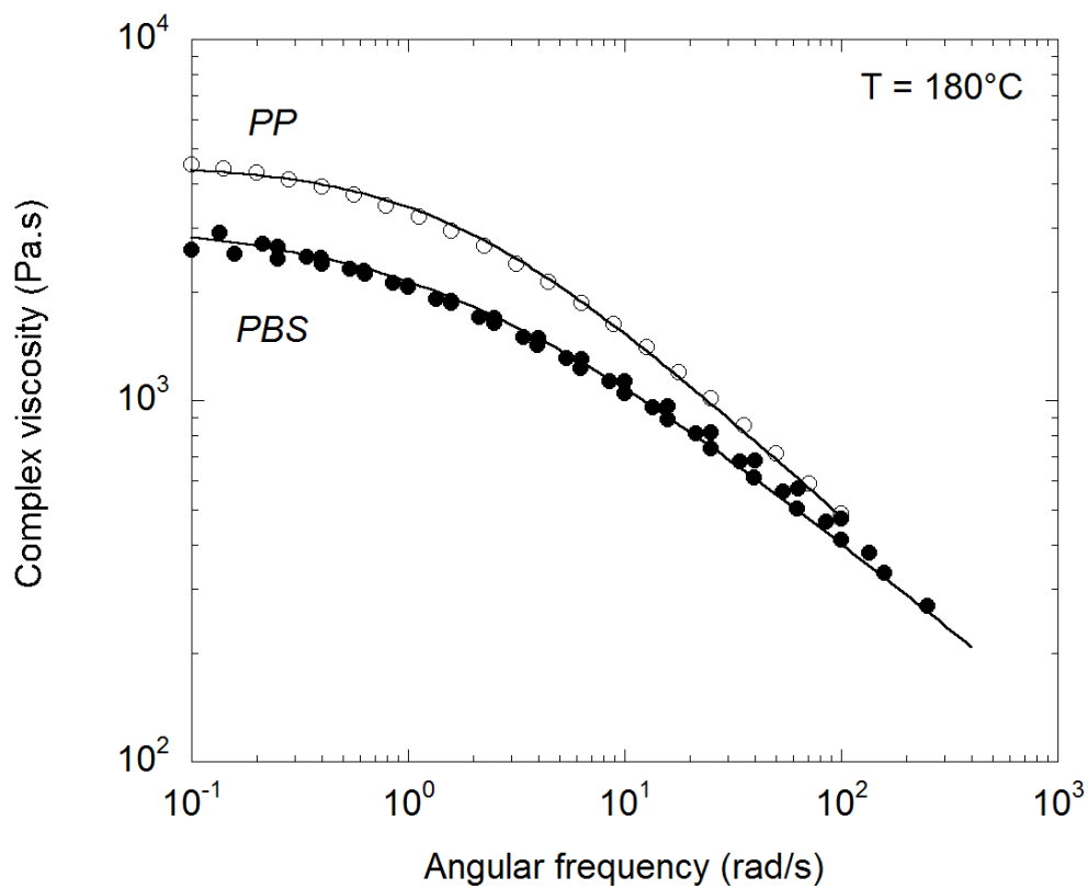
Figure 1. Complex viscosity curves of PP (with 2.5% PP-g-MA) and PBS at 180°C. Full lines are fits with the Carreau-Yasuda model.
