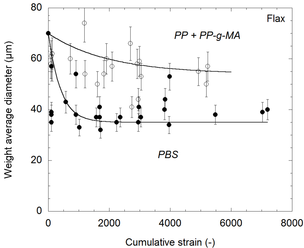
Figure 6. Changes in weight average fiber diameter as functions of the cumulative strain for various processing conditions. Full lines are fits with Eq. (2).
