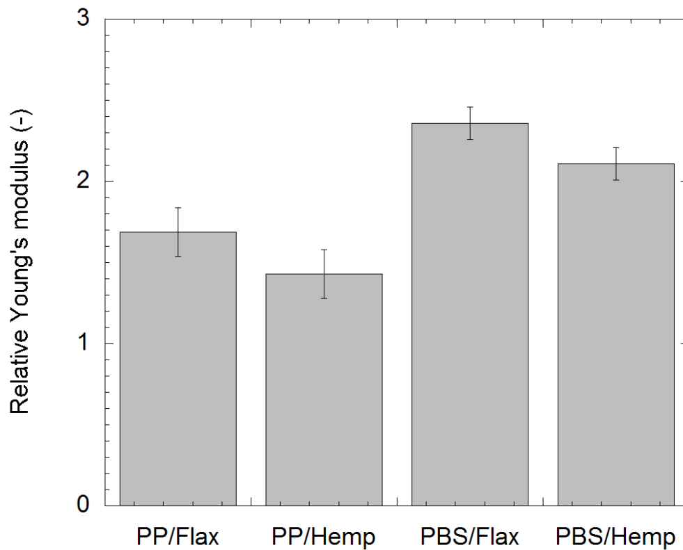
Figure 11. Mechanical properties of the various composites. (a) Relative Young's modulus, (b) Stress at break, (c) Elongation at break. PP means PP/PP-g-MA.
