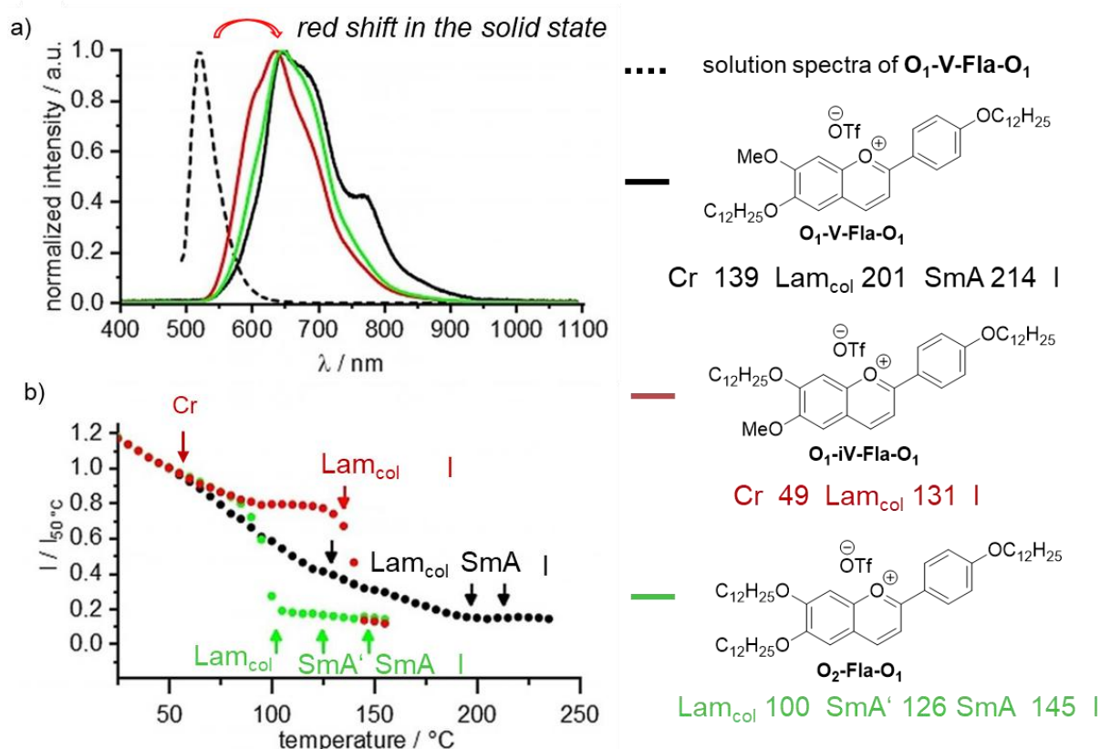
Figure 10. a) Emission spectra of O 1 -V-Fla-O 1 (black), O 1 -iV-Fla-O 1 (red) and O 2 -Fla-O 1 (green) in the solid state at 50 °C upon excitation with UV light (350 – 380 nm), solution spectrum of O 1 -V-Fla-O 1 is given in dashed lines for comparison and b) temperature-dependent emission intensity at 665 nm measured during cooling the sample from the isotropic liquid (cooling rate of 10 Kmin -1 ). For the orientation transition temperatures of the DSC are given as arrows. The figure was taken from ref. [43] and modified. This is an open access article distributed under the terms of the Creative Commons CC BY license, which permits unrestricted use, distribution, and reproduction in any medium, provided the original work is properly cited.
