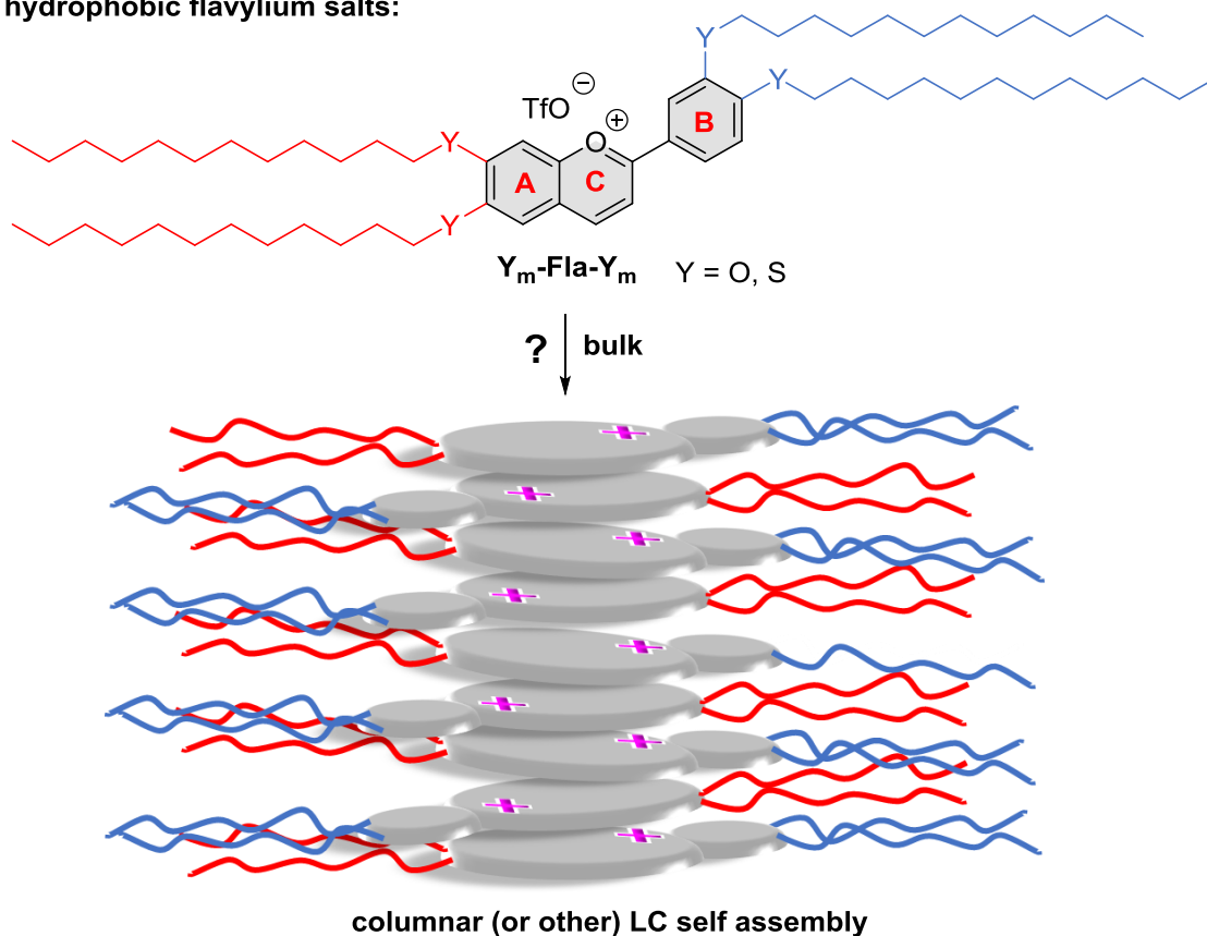
Scheme 3. Proposed bulk self-assembly of hydrophobic flavylium salts.
