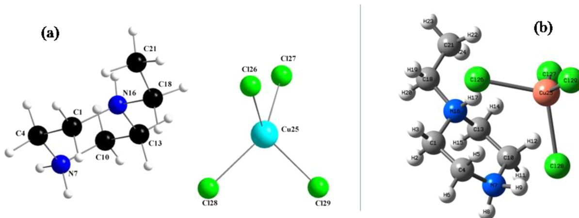
Figure 1. (a) Asymmetric unit with atom labeling and (b) optimized structure used in theoretical studies.
