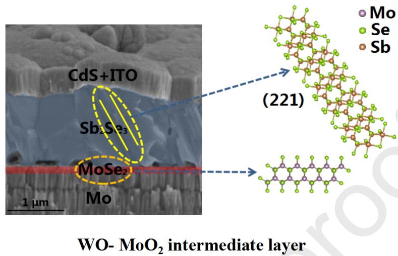
Fig. S3. Cross-sectional SEM image of S Mo1 device (WO-MoO 2 intermediate layer)
