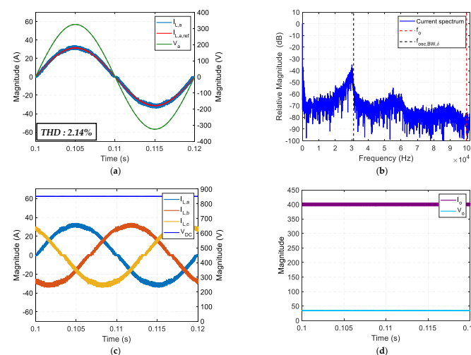
Figure 14. Waveforms of the global energy conversion chain: (a) grid voltage, grid current controlled by DPSSOCC and its reference, (b) current spectrum of the phase a, (c) input currents and DC voltage bus and (d) arc current and voltage.
