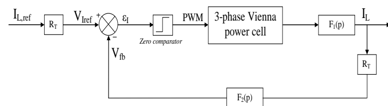
Figure 2. PSSOCC current control technique synoptic per phase.
