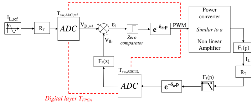
Figure 8. DPSSOCC proposed model.
