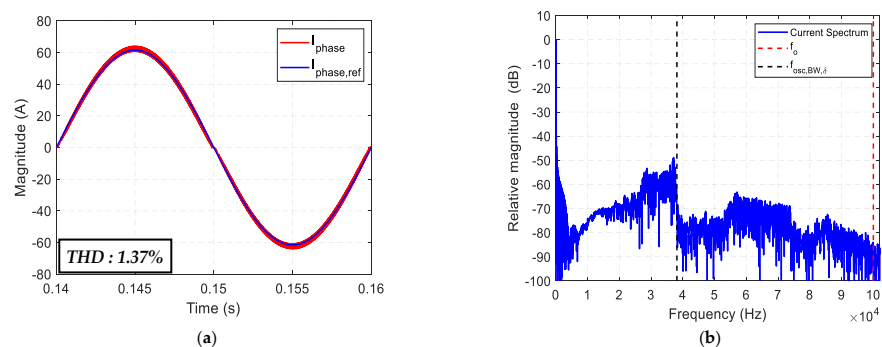
Figure 9. (a) Input current controlled by digital DPSSOCC and (b) its related current spectrum.
