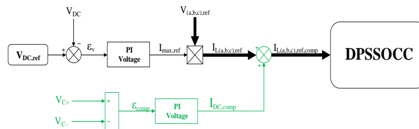
Figure 4. Synoptic of the imbalance voltage compensation loop.
