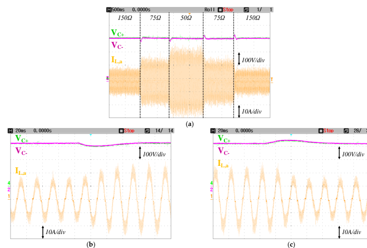
Figure 20. DPSSOCC performances with resistive load variations: (a) between 150\ \Omega and 50\ \Omega , (b) transient from 75\ \Omega to 50\ \Omega (zoom) and (c) transient from 50\ \Omega to 75\ \Omega (zoom).
