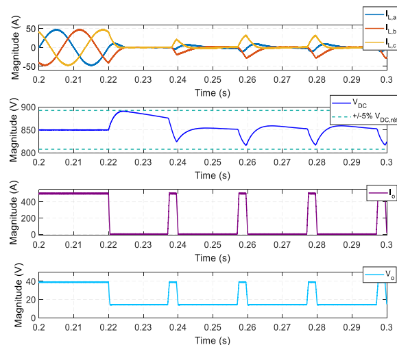
Figure 17. Waveforms in pulsed current operation mode.
