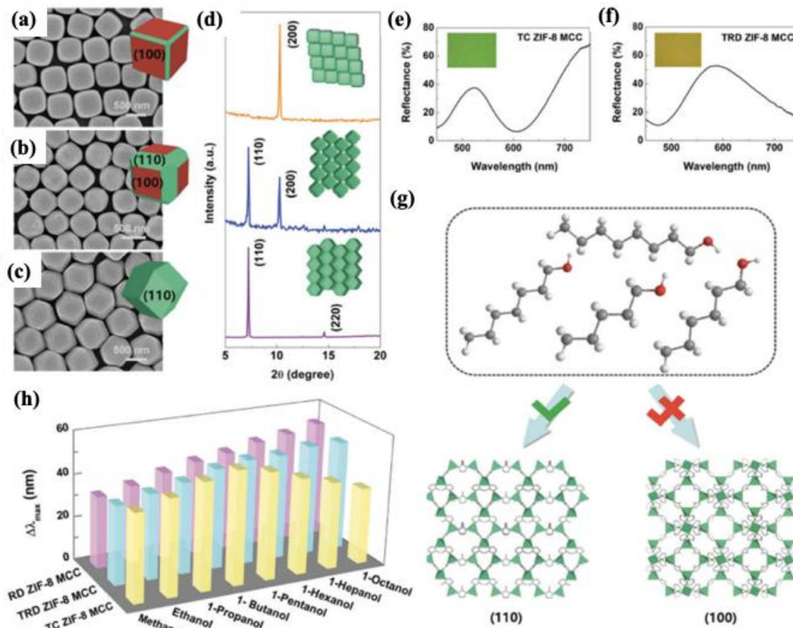
Figure 10. (a–c) SEM images of ZIF-8 MCCs of different crystal morphologies: TC ZIF-8 (a), TRD ZIF-8 (b) and RD ZIF-8 (c). Insets show schematic representations of corresponding crystal morphologies. (d) PXRD patterns of ZIF-8 MCCs of different crystal morphologies showing preferential orientations. Inset show schematic representations of corresponding arrangement of ZIF-8 nanoparticles. From top to bottom: TC ZIF-8, TRD ZIF-8 and RD ZIF-8. (e and f) Reflectance spectra of TC ZIF-8 MCCs (e) and TRD ZIF-8 MCCs (f). Insets show corresponding optical micrographs. (g) Schematics showing the adsorption of C5–C8 linear alcohols on ZIF-8 through (110) and (100) planes. (h) \Delta\lambda_{\max} of ZIF-8 MCCs of different crystal morphologies in response to C1–C8 linear alcohols: RD ZIF-8 (pink), TRD ZIF-8 (cyan) and TC ZIF-8 (yellow). 112
