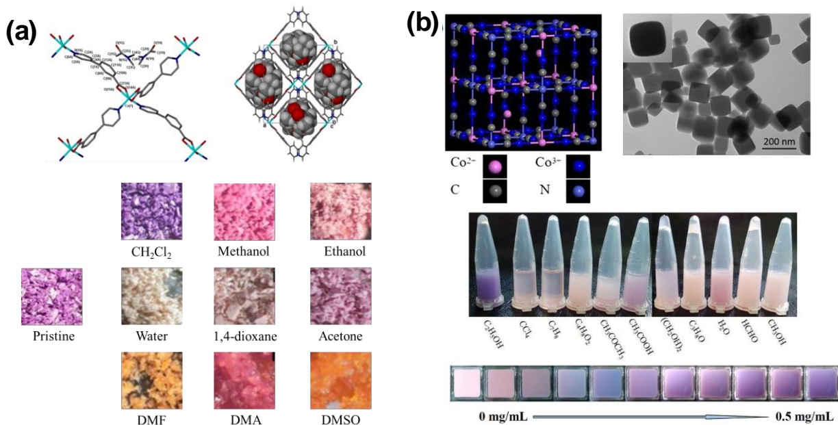
Figure 3. (a) Coordination environment of Co(II), packing of {[Co(3,4pba) 2 ·(H 2 O)]·1/2DMF·H 2 O} n ; and pictures of powered samples after exposure to different solvents. Figures adapted from ref 126. (b) Structure of Co 3 [Co(CN) 6 ] 2 , and TEM of the nanoparticles; The colour of Co 3 [Co(CN) 6 ] 2 films changes from pink to purple gradually with an increasing ethanol concentrations gradient. Adapted with permission from ref 96.
