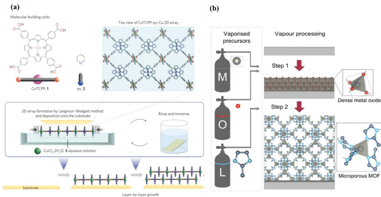
Figure 1. (a) Schematic illustration of the fabrication of NAFS-1 with bottom-up modular assembly by combining a layer-by-layer growth technique with the Langmuir-Blodgett method. Reproduced from ref 78 . (b) Vapour-phase deposition of ZIF-8 thin films via ALD ZnO film. The procedure consists of a metal oxide vapour deposition (Step 1) and a consecutive vapour-solid reaction (Step 2). Metal, oxygen and ligand sources are labelled as M, O and L, respectively. Metal oxide deposition can be achieved by atomic layer deposition (M, diethylzinc; O, oxygen/water) or by reactive sputtering (M, zinc; O, oxygen plasma). Atom colours: zinc (grey) oxygen (red), nitrogen (light blue) and carbon (dark blue); hydrogen atoms are omitted for clarity. Illustration reproduced from Ref 78.
