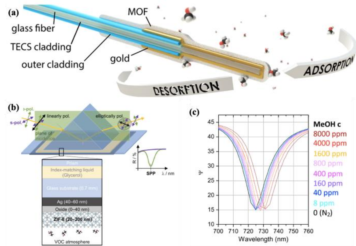
Figure 14. (a) Schematic representation of an MOF-FO-SPR probe (not in real scale). The probe consists of an optical fibre with a diameter of 400 \mu\text{m} with the inner TECS cladding and the outer protective cladding removed from the end. A gold layer is covered with a MOF which functions as a recognition layer. The atoms in the floating methanol molecules are oxygen (red), carbon (black), and hydrogen (white). 120 (b) TIRE/SPP principle and TIRE measurement geometry with the sample layer stacks. (c) The measured SPP peak redshift under Methanol in dry \text{N}_2 . 121
