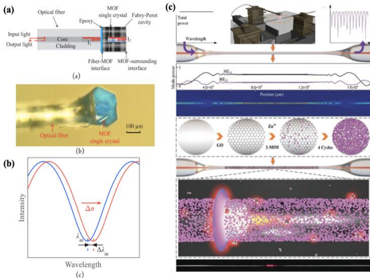
Figure 12. (a) Schematic diagram of the HKUST-1 coated optical fibre sensor and an optical microscope image of the sensor. (b) Illustration of a section of the original (blue) and shifted (red) interferograms. 180 (c) Schematics of the modification step at the interface of the optical microfiber with ZIF-8/GO functional layer. 118
