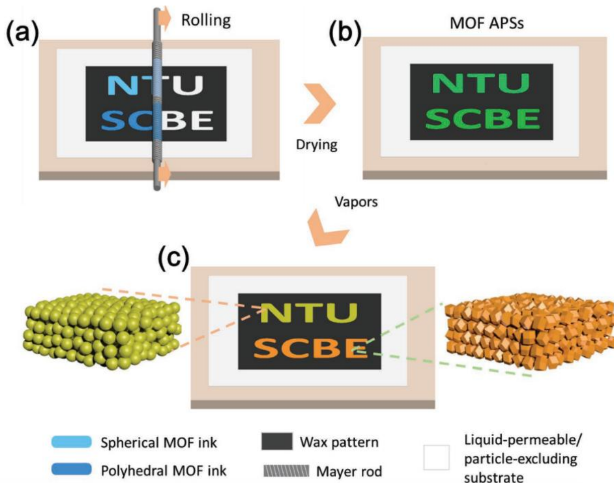
Figure 11. Illustration of Mayer rod coating of MOF amorphous photonic structure (APS). (a) Selective wetting of the hydrophilic area of the substrate during coating by spherical/polyhedral MOF inks; b) Formation of APS patterns of spherical or polyhedral MOF particles after the removal of water; c) Vapour-responsive colour changes of the MOF APS patterns. 175
