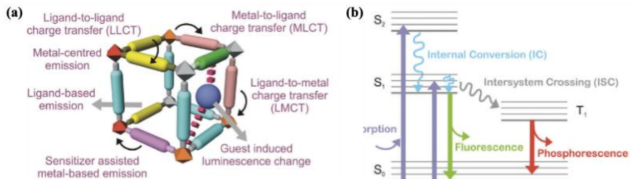
Figure 6. (a) Schematic diagram of various origins of luminescence in LMOFs. (b) Illustration of photon emission in ligand-centred luminescence. Adopted from ref 151.
