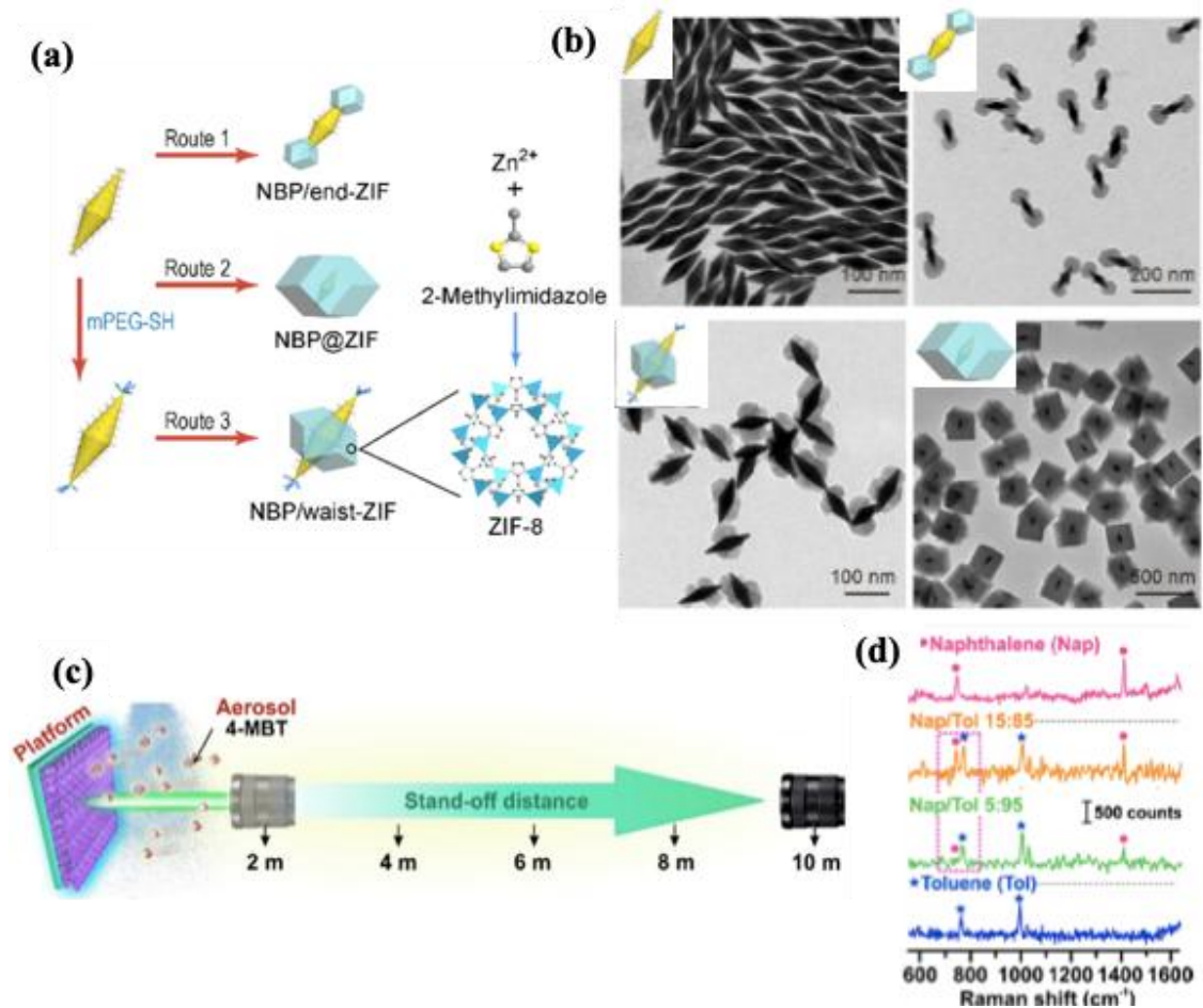
Figure 15. (a) Schematics of the routes for selective deposition of ZIF-8 on the Au NBPs. (b) TEM images of the Au NBPs, NBP/end-ZIF, NBP/waist-ZIF, and NBP@ZIF nanostructures, respectively. 194 (c) Illustration of the setup for stand-off SERS sensing. (d) Stand-off multiplex spectra obtained in outdoor condition with natural light, for two different mixtures of naphthalene and toluene, with reference to individual naphthalene and toluene SERS spectra.
