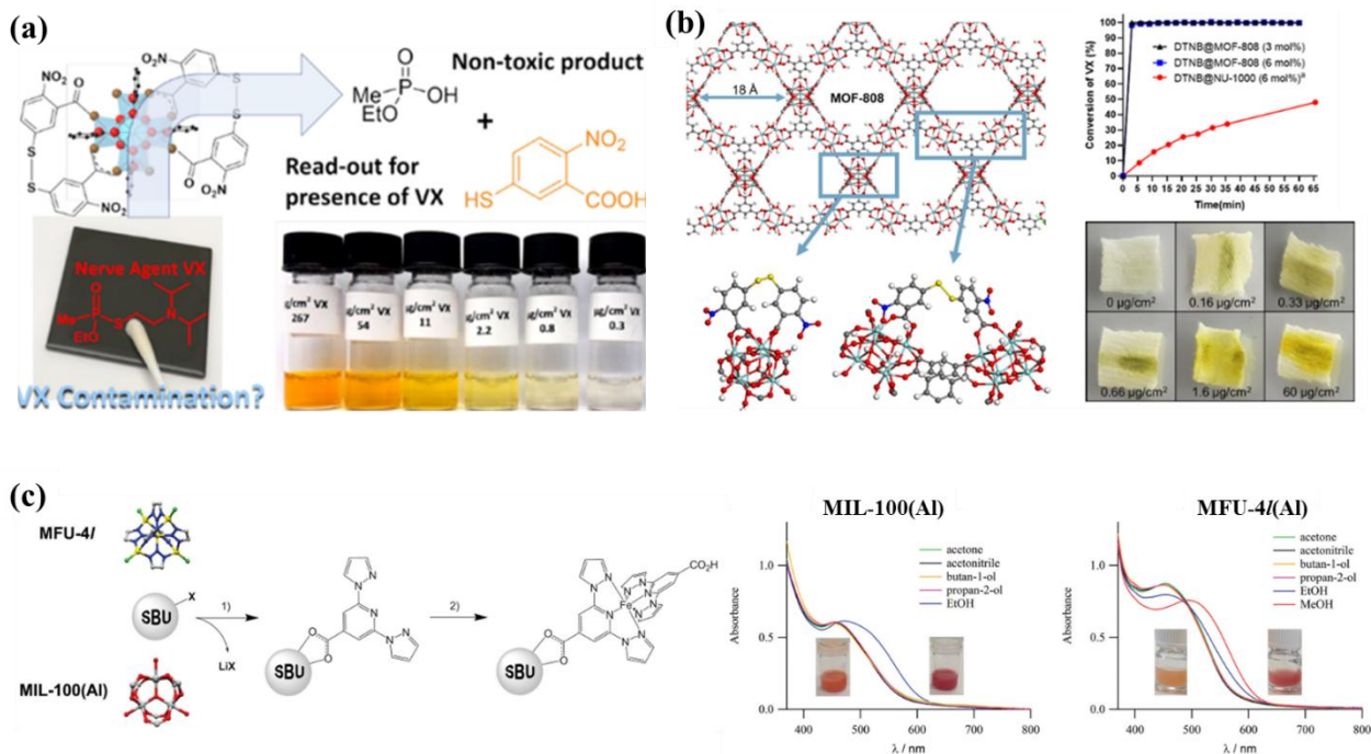
Figure 5. (a) Illustration of DTNB@NU-1000 for degradation and visual detection of the nerve agent VX. 143 (b) Two anchoring modes of DTNB in MOF-808 and the proposed mechanism of the colour change of DTNB@MOF-808 upon VX. DTNB@MOF-808 degradation kinetics of VX compared to DTNB@NU-1000. Photographs of the MOF-textile composite upon contact with VX. 144 (c) Sequential installation strategy for anchoring a SCO complex in a MOF and UV-Vis spectra at room temperature of the MOF-SCO composites dispersed in acetone (orange) and EtOH (red) for MIL-100, and dispersed in acetone (orange) and MeOH (red) for MFU-4l. 106
