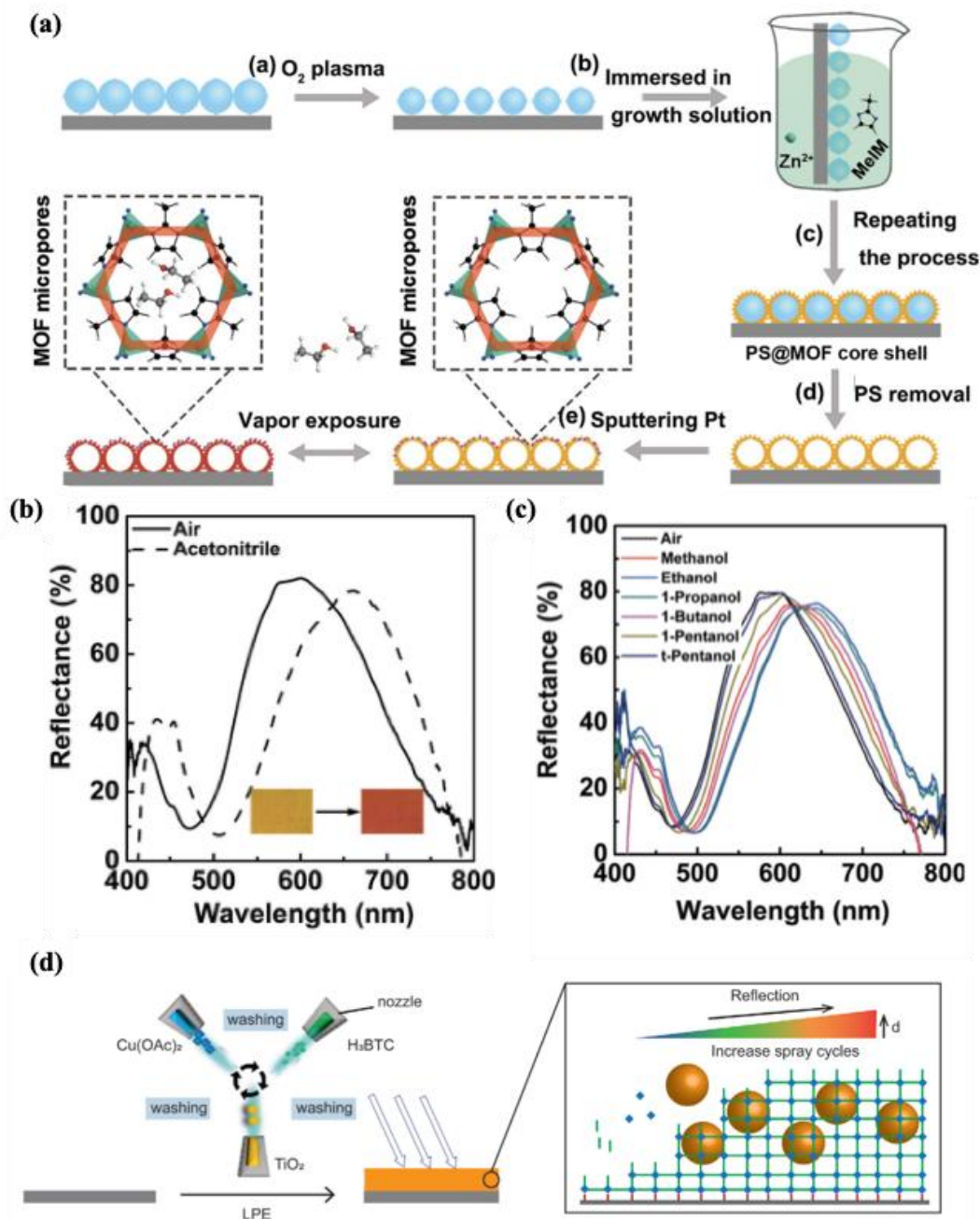
Figure 9. (a) Illustration of the experimental procedure used to fabricate HMNSE. (b) HMNSE with 2 nm Pt coating before and after exposure to a saturated acetonitrile vapour at 293 K. Insets are corresponding optical microphotographs. (c) Optical response of HMNSE to different alcohols, including methanol, ethanol, 1-propanol, 1-butanol, 1-pentanol, and tert-pentanol. 110 (d) Schematic of the liquid phase epitaxy (LPE) method for sequential TiO_2 -loading in MOF films. 111
