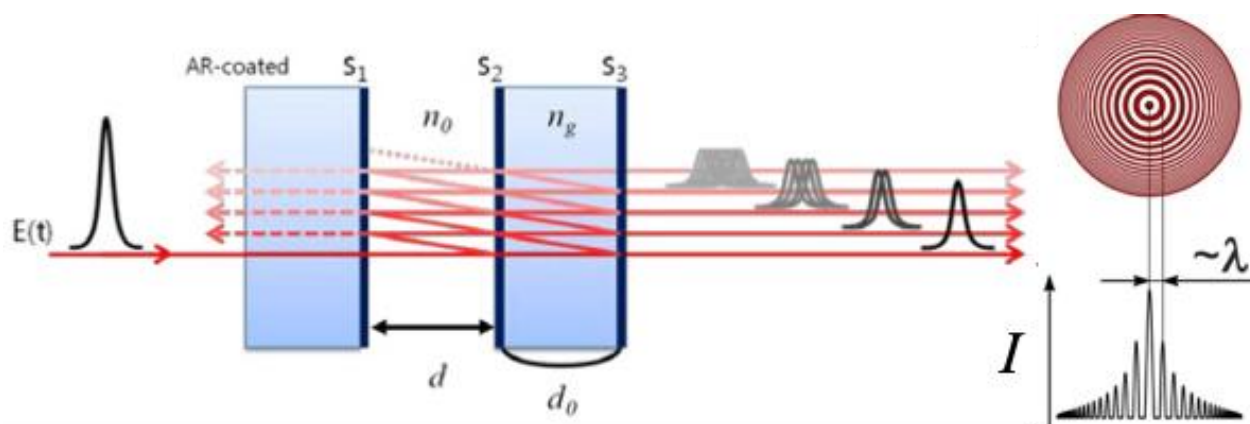
Figure 8. Illustration of the working principle of a Fabry-Perot interferometer and a typical Fabry-Perot interference pattern.
