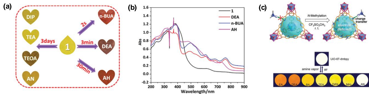
Figure 4. (a) Color change and response time of [\text{Zn}(\text{3-DPMNI})_{0.5}(\text{NDC})] (denoted as 1 in the figure and following text), ( \text{H}_2\text{NDC} = 2,6-naphthalenedicarboxylic acid, 3-DPMNI = N,N' -bis(3-pyridylmethyl)-1,4,5,8-naphthalene diimide) in the presence of different amine vapors. (b) UV-vis absorption spectra of 1 in the presence of different organic amines. Figures adapted from ref 105. (c) Structure of N-methylated UiO-67-bpy and its reversible colour change when deposited UiO-67-dmbpy was exposed to amine vapours. n-BUA(in a)/BA (in c) = butylamine, DEA = diethylamine, AH = hydrazine, DIP(in a)/DiPA (in c)= diisopropylamine, TEA = triethylamine, TEOA = triethanolamine, AN = aniline, EA = ethylamine. Figures adapted from ref 100.
