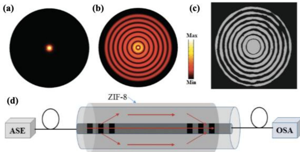
Figure 13. (a) Optical power distribution of the fundamental mode ( LP_{01} , core mode) and (b) higher-order mode ( LP_{08} , cladding mode); (c) near-field image of the LP_{08} mode pattern obtained with an infrared camera; (d) schematic diagram of the proposed fibre interferometer with cascaded LPFGs. ASE: amplified spontaneous emission light source; OSA: optical spectrum analyzer. 119
