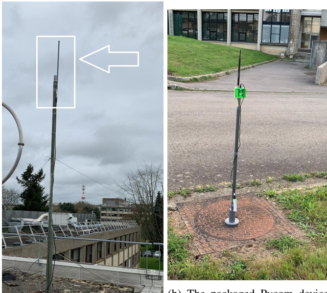
(a) The gateway monopole antenna connected to the cable. (b) The packaged Pycom device fixed on a rod and connected to a battery at location 4.
