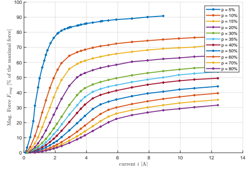
Fig. 2. Experimental characterization of F_{mag} with respect to the current i and the airgap p (as a percentage of the maximal displacement).
