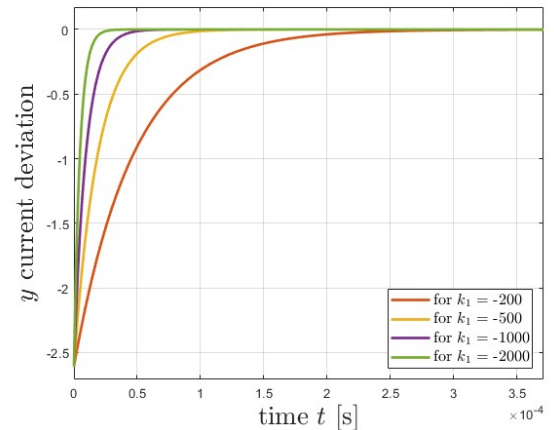
Fig. 5. Plot of the current deviation w.r.t. the suitable current for the desired mechanical dynamic y = i - i_a .
