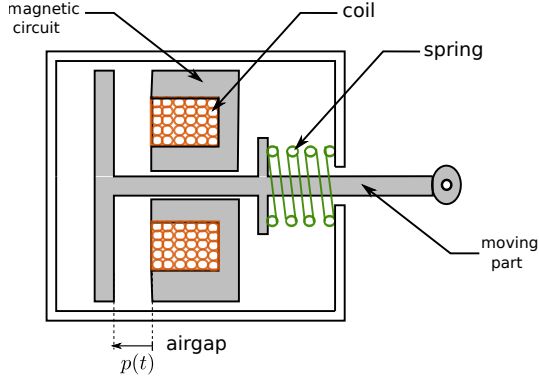
Fig. 1. Scheme of the actuator.
