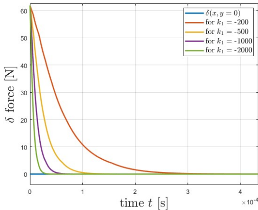
Fig. 6. Plot of the force deviation \delta(x, y) .
