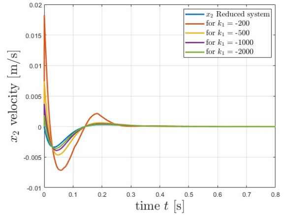
Fig. 4. Plot of the velocity x_2 = v .
