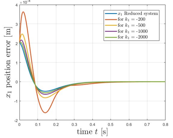
Fig. 3. Plot of the position deviation w.r.t. the reference x_1 = p - r .
