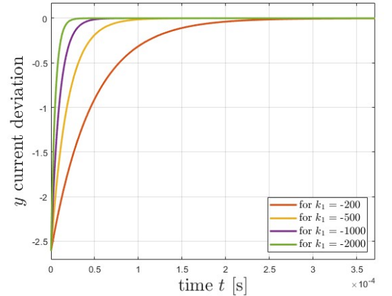
Fig. 5. Plot of the current deviation w.r.t. the suitable current for the desired mechanical dynamic y = i - i_a .
