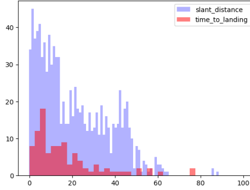
Figure 7: Comparison of distance estimation between real images and synthetic images in the test set
