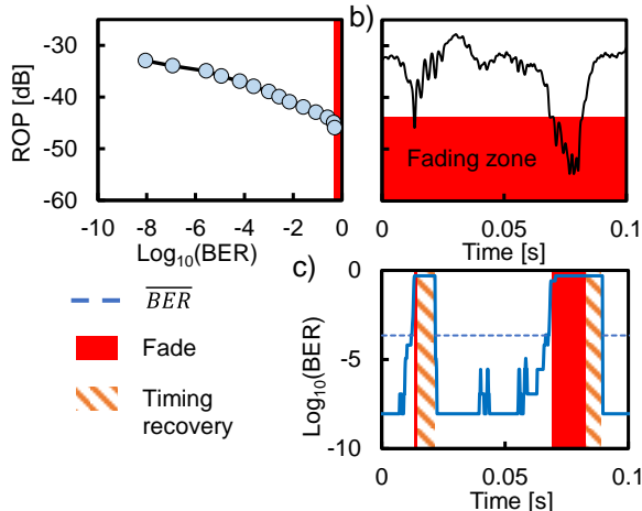
Fig.3: (a) The dependence of the measured BER with ROP. BER reaches 0.5 for ROP <-45 dBm (b) A snippet of a time series of 100 ms with the fading zone in red. (c) BER of the time series.
