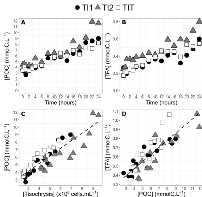
Figure 3. Particulate organic carbon (POC) concentration (A) of the two enriched balloons of Tisochrysis lutea (TI1 and TI2, filled black circles and filled gray triangles, respectively) and of the control balloon (TIT, empty squares) and total fatty acids (TFA) concentration according to culture age in hours (B). POC concentration according to algae concentration (C). Relation between total fatty acids and POC concentration (D). All regressions (dotted lines) have been calculated with data from the three balloons combined together.
