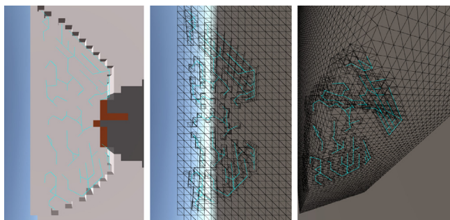
Fig. 9. 3D view of a cracked wall, where the voxels were displaced in a similar way as in Fig. 6. The cracks are represented with cyan lines. Whenever possible, we join and merge the cracks. From left to right: lateral “voxel view” of a wall segment, cracks inside the material with voxel silhouettes, and 3D view of the cracks inside the material where we can see them gathering together.
