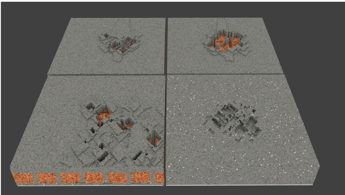
Fig. 15. Ice formation on a layer of plaster lying on top of bricks, from left to right and top to bottom: (1) a small rain area; (2) small rain density area under a longer exposure; (3) same exposure but with a larger area; (4) a wall with plaster only.
