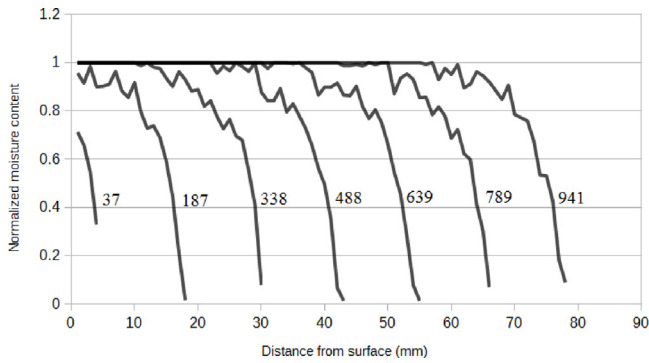
Fig. 7. Curves representing the Volume Fractional Saturation (VFS) obtained with our particle-based simulation at different time steps for a wall made of concrete. The moisture advance depends on the material's water saturation.
