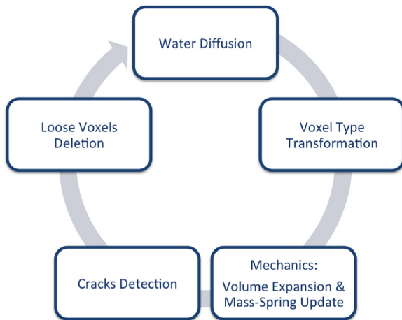
Fig. 3. Overview of the simulation loop.
