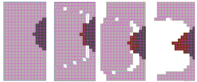
Fig. 6. A schematic 2D example of a rusting pipe inside a wall. Forces are represented as strings (purple lines) that propagate stress among the voxels. Cracks lines are shown (in cyan), as well as iron voxels (in dark gray), wall material voxels (plaster or concrete, in light gray), and rust voxels (in dark red). From left to right: the pipe in its initial state inside the wall material. As rust appears to occupy a larger volume, material voxels are pushed over and fall off.
