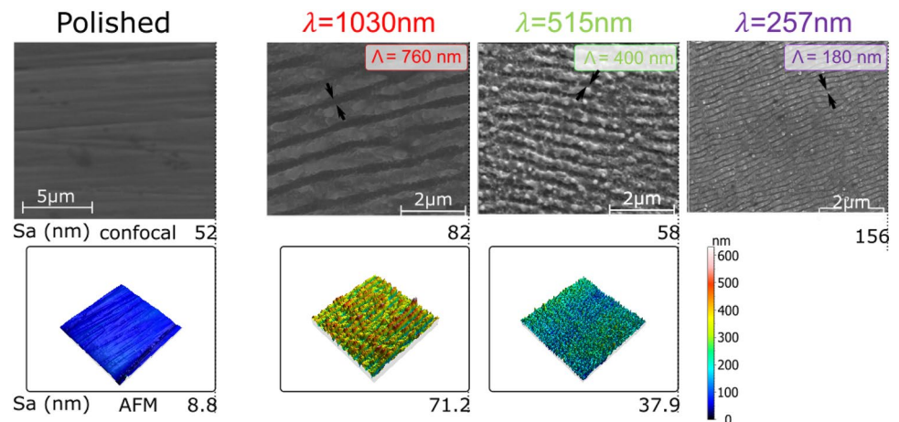
Fig. 2 SEM images and AFM surface profile of polished Ti6Al4V surface (left) and LIPSS induced at different wavelengths (right). Their ripple periodicity \Lambda and arithmetical mean height ( S_a ) measured by confocal microscope and AFM are shown above and below the images respectively
