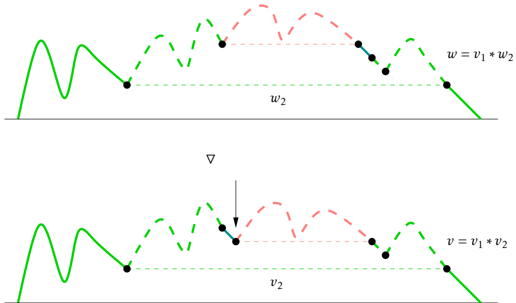
FIGURE 7. Second type of cover relation v \triangleleft w when v = v_1 * v_2 . The cover relation involves a down step of v_2 .
