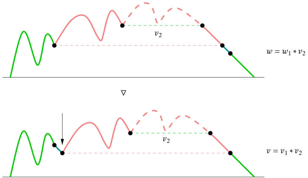
FIGURE 6. First type of cover relation v \triangleleft w when v = v_1 * v_2 . The cover relation involves a down step of v_1 .
