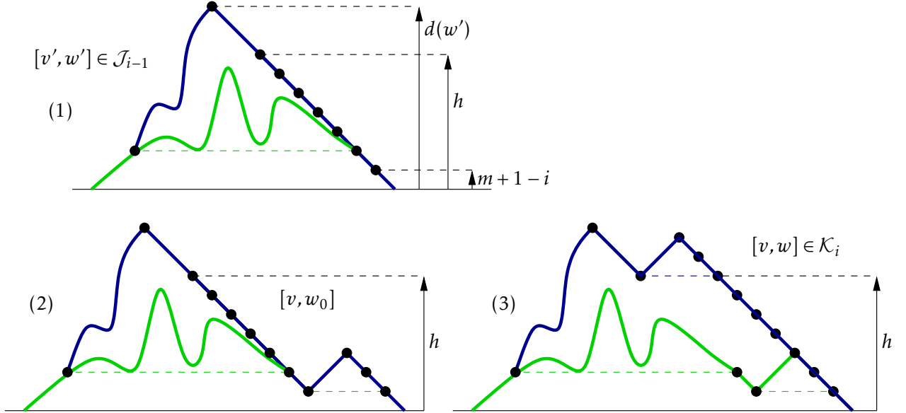
FIGURE 10. From an interval [v', w'] in \mathcal{J}_{i-1} and a height h in \llbracket m + 1 - i, d(w') \rrbracket to an interval [v, w] in \mathcal{K}_i . Here, m = 2 , i = 2 and h = 7 .
