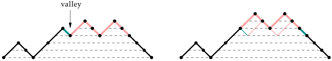
FIGURE 1. Example of greedy cover relation, with n = 5 and m = 2 .
