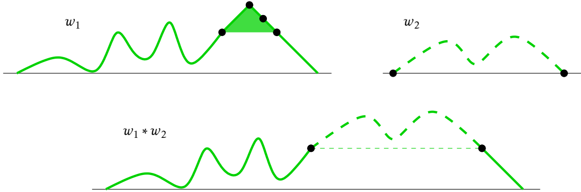
FIGURE 5. The monoid structure on m -Dyck paths, when m = 2 .
