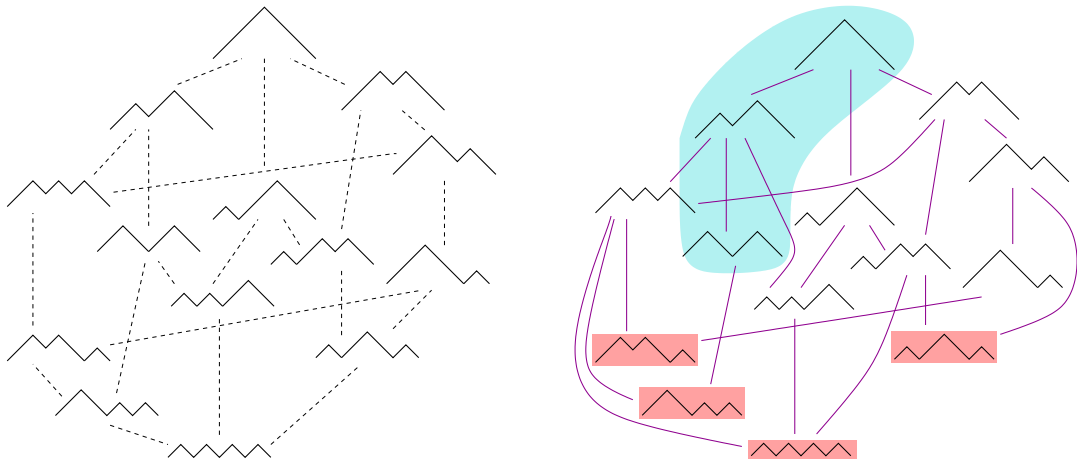
FIGURE 3. The ordinary Tamari lattice on \mathcal{D}_{1,n} with n = 4 (left), and its greedy counterpart (right). The chain above 11001100 is order-isomorphic to the greedy order on \mathcal{D}_{2,2} .
