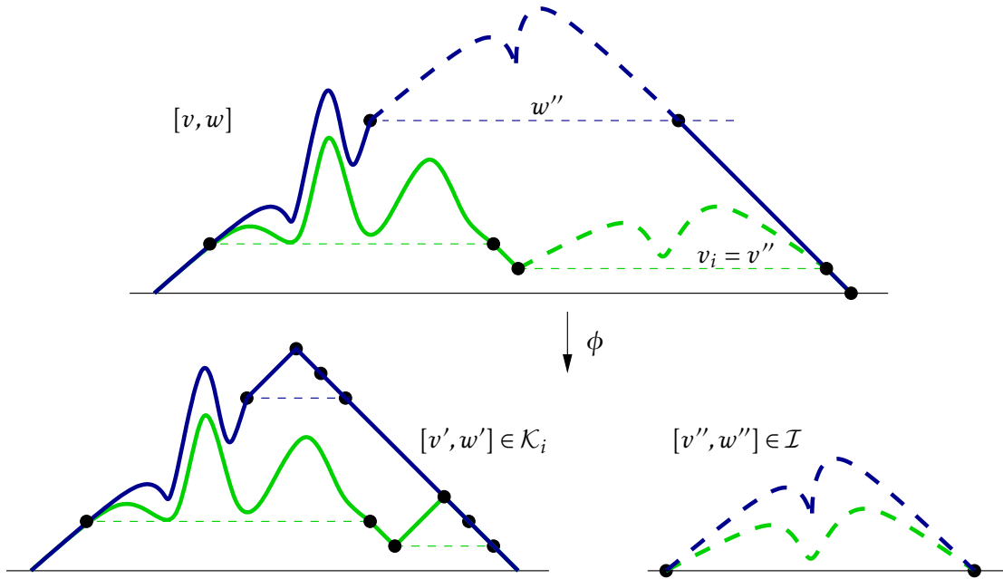
FIGURE 9. Decomposition of an interval [v, w] of \mathcal{J}_i \setminus \mathcal{J}_{i-1} , with m = 2 and i = 2 .
