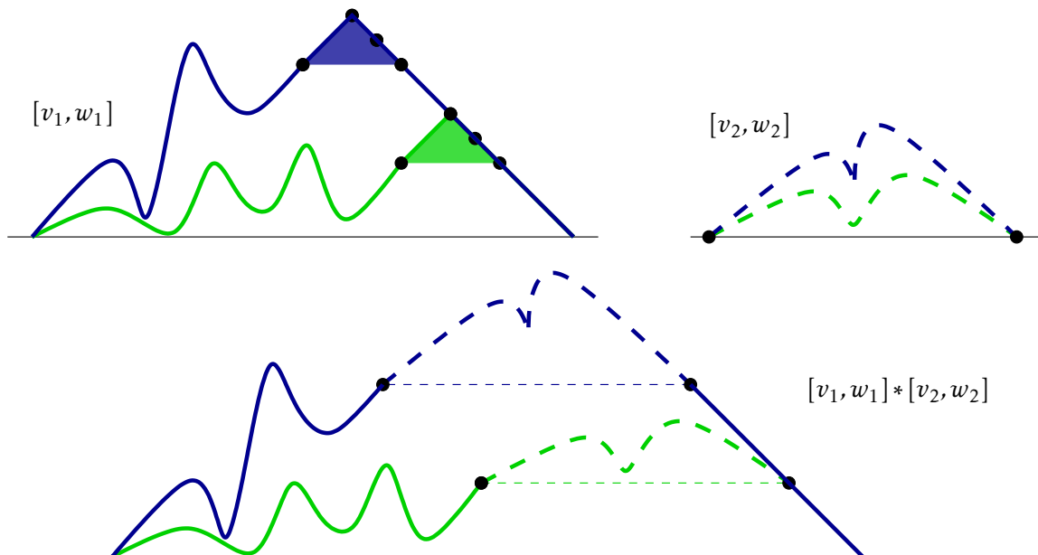
FIGURE 8. The monoid structure on greedy intervals, when m = 2 .
