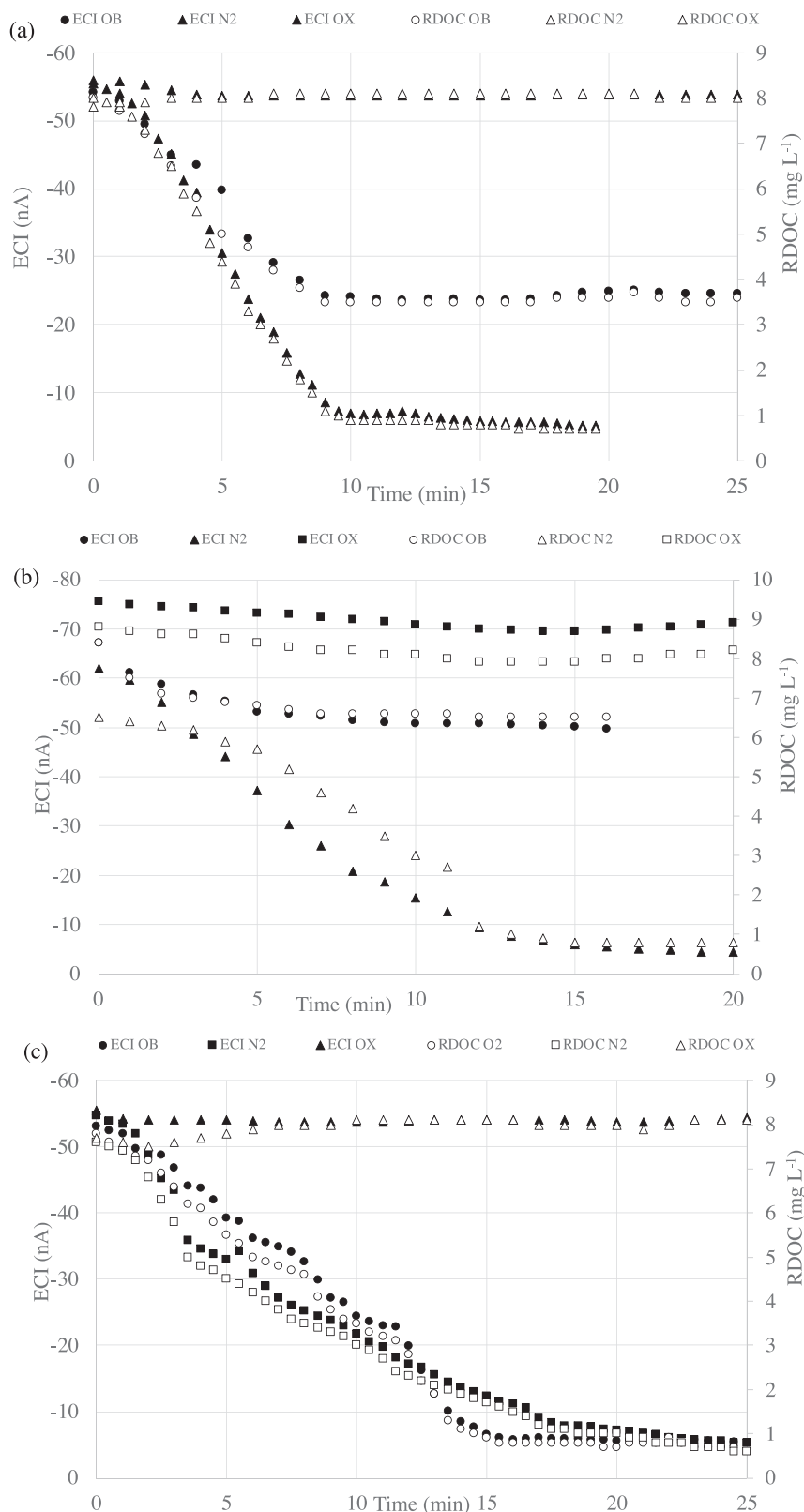
Figure 7. Variations of ECI and RDOC as a function of time for three different vegetable oils: a) peanut; b) rapeseed; c) sunflower. OB: bottle opening, N 2 : degassing by bubbling nitrogen, O 2 : oxygenation by bubbling air.
