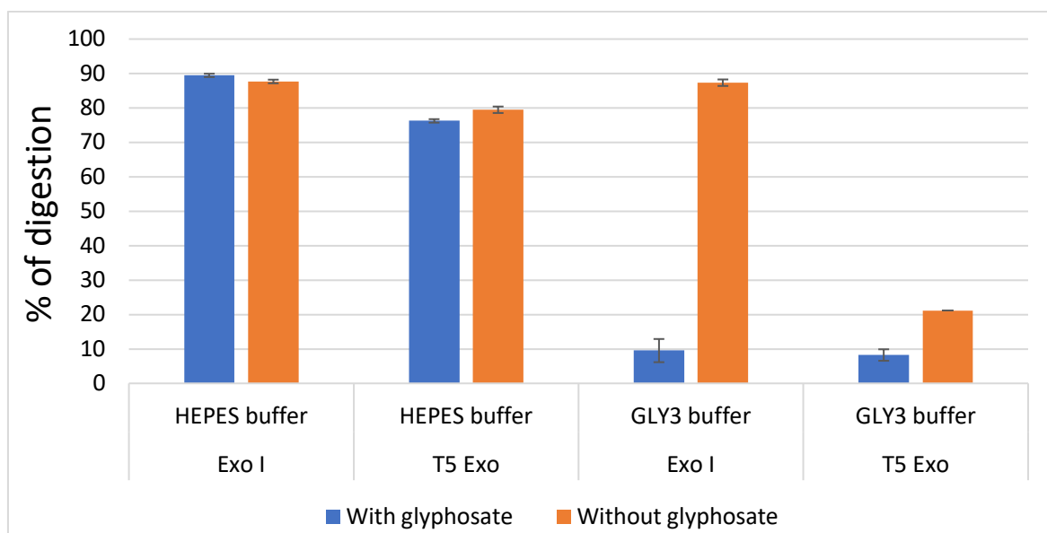
11 Figure 4. Digestion of SUP000 (1 μM), Exo I and T5 Exo, for 30 min at 37 °C in HEPES and 12 GLY3 buffers with and or glyphosate (1 mM). 13
