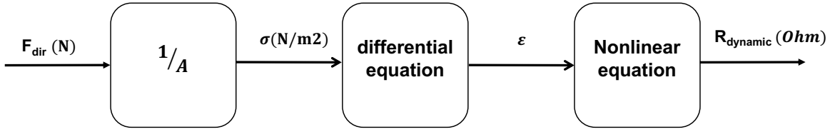
Fig. 11. The direct model of resistance R_{dynamic} as a function of force F_{dir} , where R_{dynamic} denotes the resistance estimated by this model, \varepsilon the strain, \sigma the mechanical stress, and F_{dir} the force measured by a test bench.
