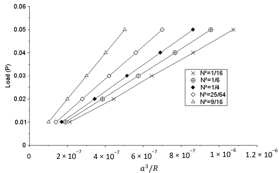
Figure 1. Plots of load ( P ) versus ( a^3/R ) for different values of the coupling number N^2 .
