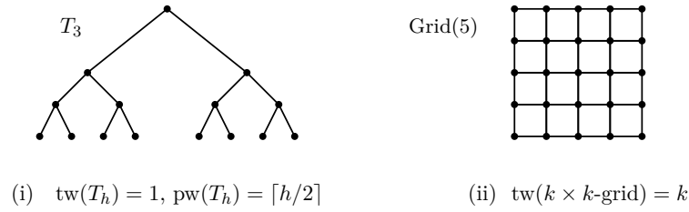
■ Figure 15 (i) The complete binary tree T_h of height h has pathwidth \lceil h/2 \rceil , cf. [11, Theorem 67]. (ii) The k \times k grid graph is known to have pathwidth and treewidth both equal to k .
