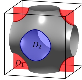
(c) Two essential disks D_i \subset \mathcal{H}_i ( i = 1, 2 ) witnessing the weak reducibility of (\mathcal{H}_1, \mathcal{H}_2, \mathcal{S}) .
