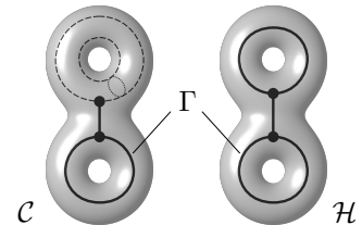
■ Figure 4 Spines of a compression body \mathcal{C} and of a handlebody \mathcal{H} .
