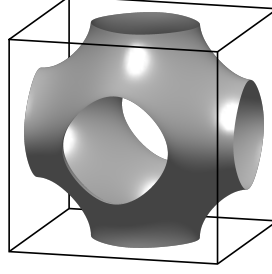
(b) A surface \mathcal{S} \subset \mathbb{T}^3 defining a Heegaard splitting (\mathcal{H}_1, \mathcal{H}_2, \mathcal{S}) of \mathbb{T}^3 of minimum genus three.
