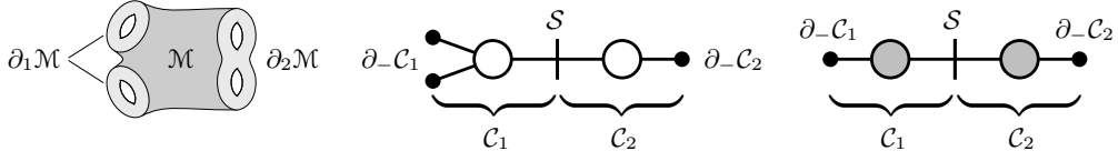
■ Figure 7 Schematic of a 3-manifold M with a partition of its boundary components (left). Faithful (center) and non-faithful (right) fork complexes representing a Heegaard splitting of (M, \partial_1 M, \partial_2 M) .
