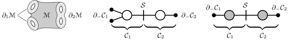
■ Figure 7 Schematic of a 3-manifold \mathcal{M} with a partition of its boundary components (left). Faithful (center) and non-faithful (right) fork complexes representing a Heegaard splitting of (\mathcal{M}, \partial_1\mathcal{M}, \partial_2\mathcal{M}) .
