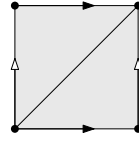
■ Figure 13 Minimal triangulation of the torus \mathbb{T}^2 .
