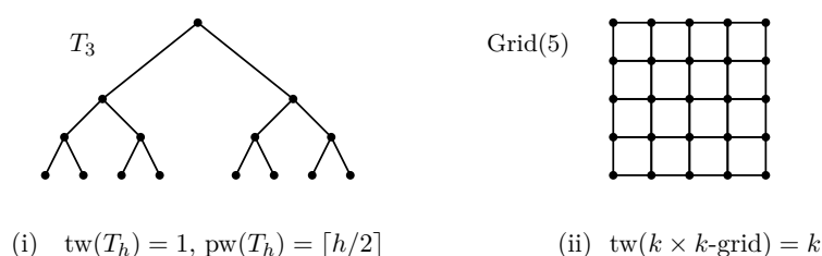
■ Figure 15 (i) The complete binary tree T_h of height h has pathwidth \lceil h/2 \rceil , cf. [11, Theorem 67]. (ii) The k \times k grid graph is known to have pathwidth and treewidth both equal to k .
