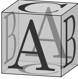
(a) The 3-torus \mathbb{T}^3 = \mathbb{S}^1 \times \mathbb{S}^1 \times \mathbb{S}^1 can be obtained by identifying opposite faces of a solid cube.
