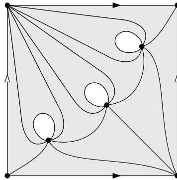
■ Figure 18 A minimal triangulation of \mathbb{T}_k^2 with 3k+2 triangles, drawn for k=3 . The extension of the drawing for larger k is straightforward.
