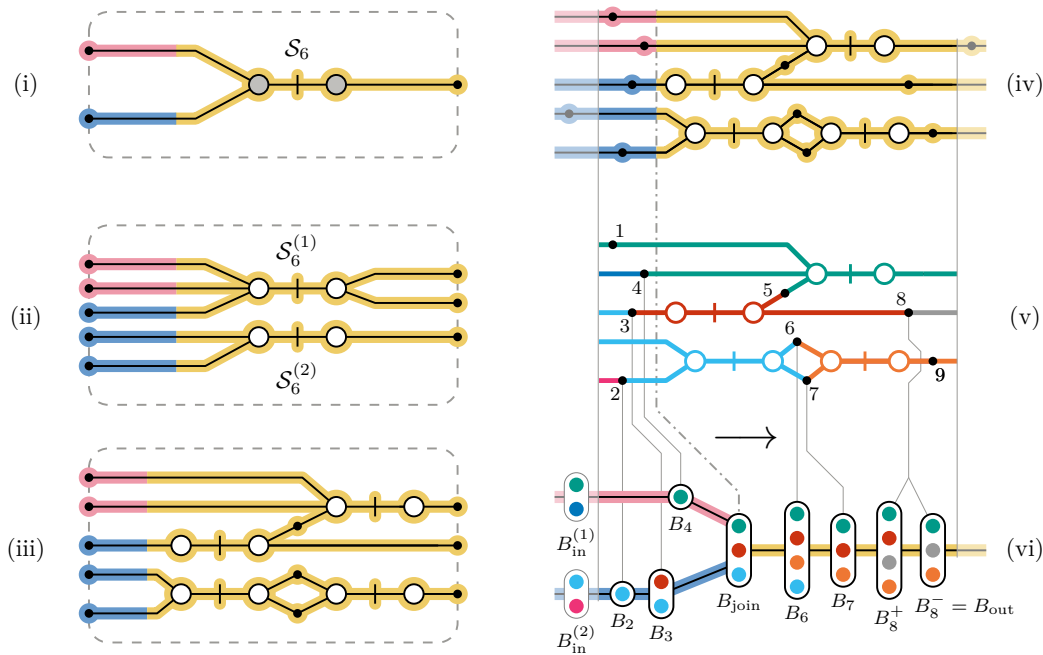
■ Figure 11 Overview of the proof of inequality (1). The figure shows the circled area in Figure 10(ii). Stage 1: Construction of initial fork complex (i) and split into faithful fork complex (ii). Stage 2: Weak reductions (iii), see [49, Proposition 5.2.3, Figures 5.8–5.13] for a complete list and their effects on the underlying fork complexes. Stage 3: perturbations and isotopy (iv). Stage 4: Construction of tree decomposition (v) and (vi).
