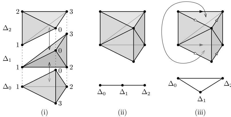
■ Figure 19 (i) The triangular prism (the shape described as t \times [0, 1] , where t denotes a triangle) can be triangulated with three tetrahedra. (ii) A triangulation of the triangular prism and its corresponding dual graph. (iii) A triangular prism with its top and bottom triangles identified. Reproduced from [27, Figure 13].
