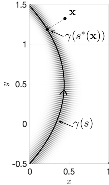
FIGURE 2. A Gaussian beam starting at (x, y) = (0, -0.5) with direction \eta_0 = \sin \Theta = 3/4 . The central ray \gamma is indicated with a solid line.
