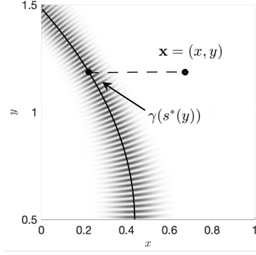
FIGURE 3. The simplified map s^*(y) .
