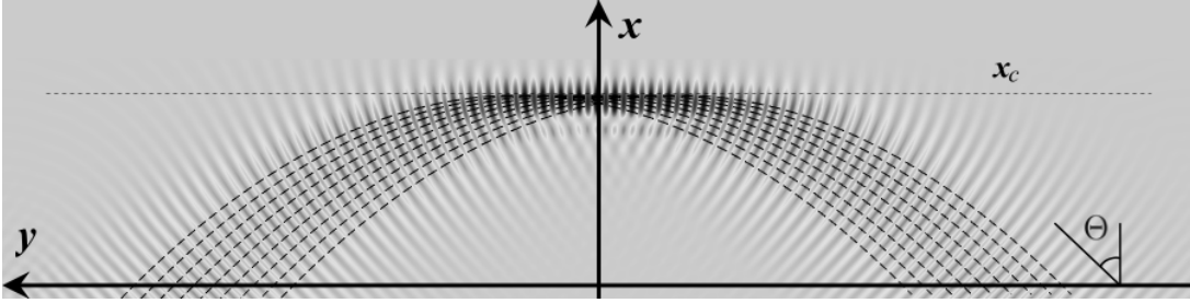
FIGURE 1. The fold caustic: Example of solution with ray tracing picture for 0 \leq x \leq 1 .
