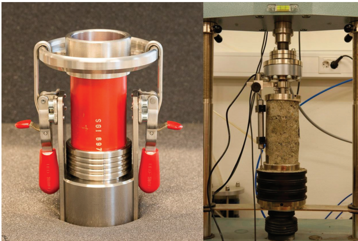
Fig. 1 Left: Photo showing packaging equipment for packing specimens with a height of 100 mm. Right: UCS testing apparatus showing a specimen after the UCS test. Photo source: Per Lindh
