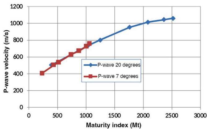
Fig. 12 P-wave versus the maturity number for soil samples cured at different temperatures.
