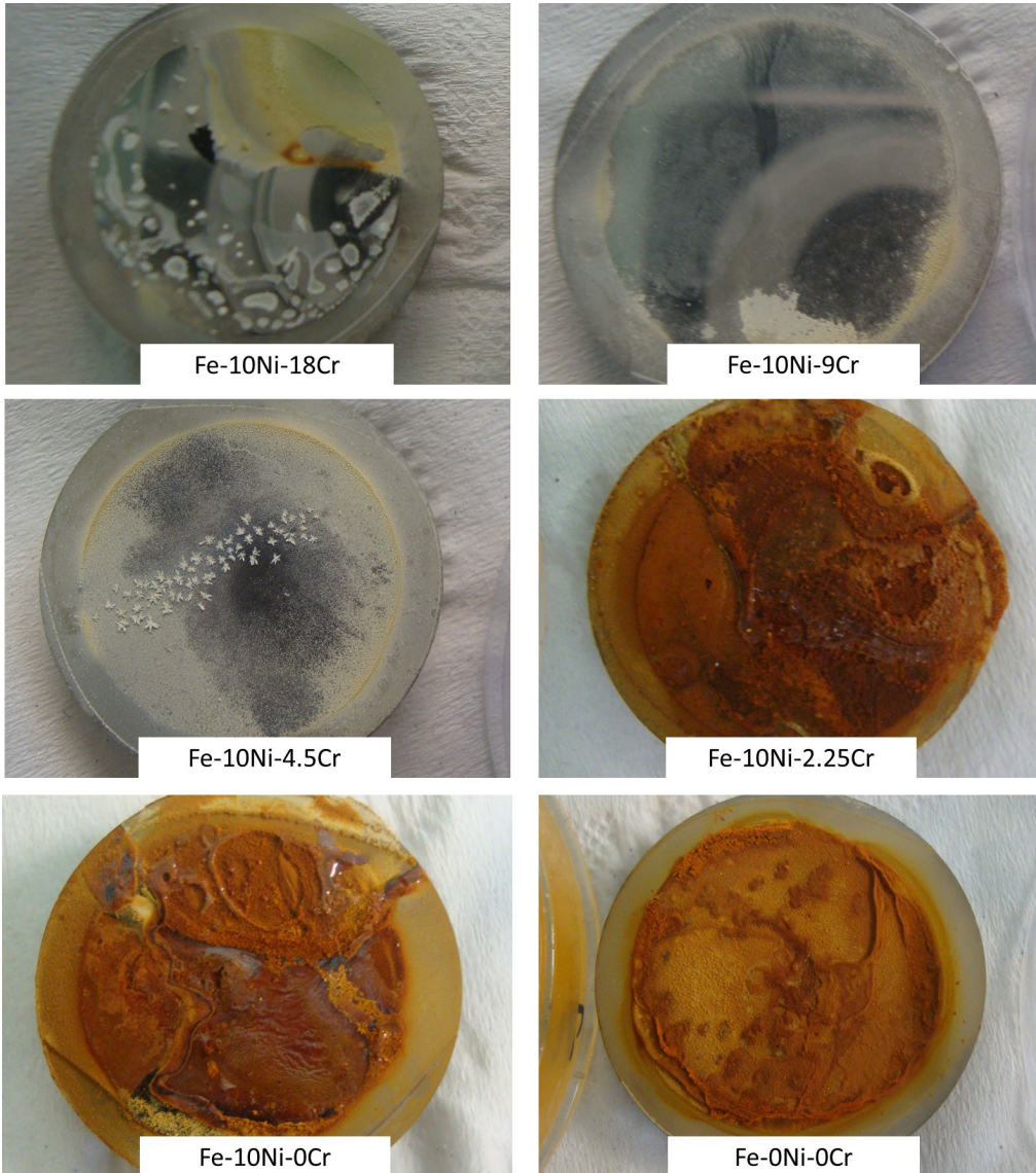
Figure 14. Final surface states of the samples after one month of immersion in Fusayama's saliva (37°C).
