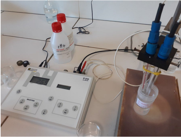
Figure 6. pH control of the solution of each cell in which one of the samples will be immersed.
