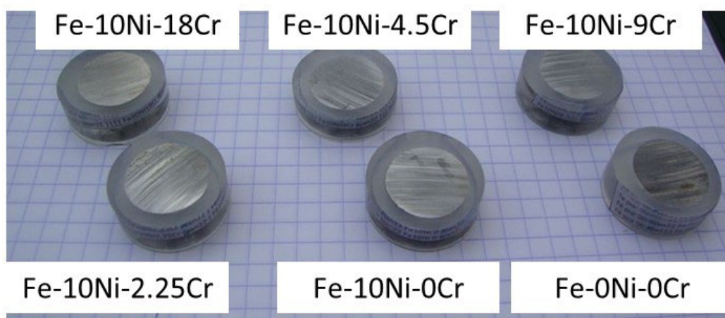
Figure 4. The part per cut embedded ingot which was devoted to the corrosion tests.
