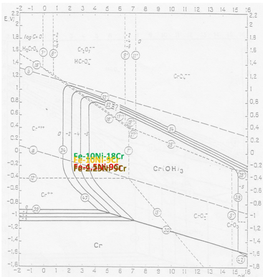
Figure 12. Positions of the last recorded values of the free potential in the Pourbaix's diagram of Cr.
