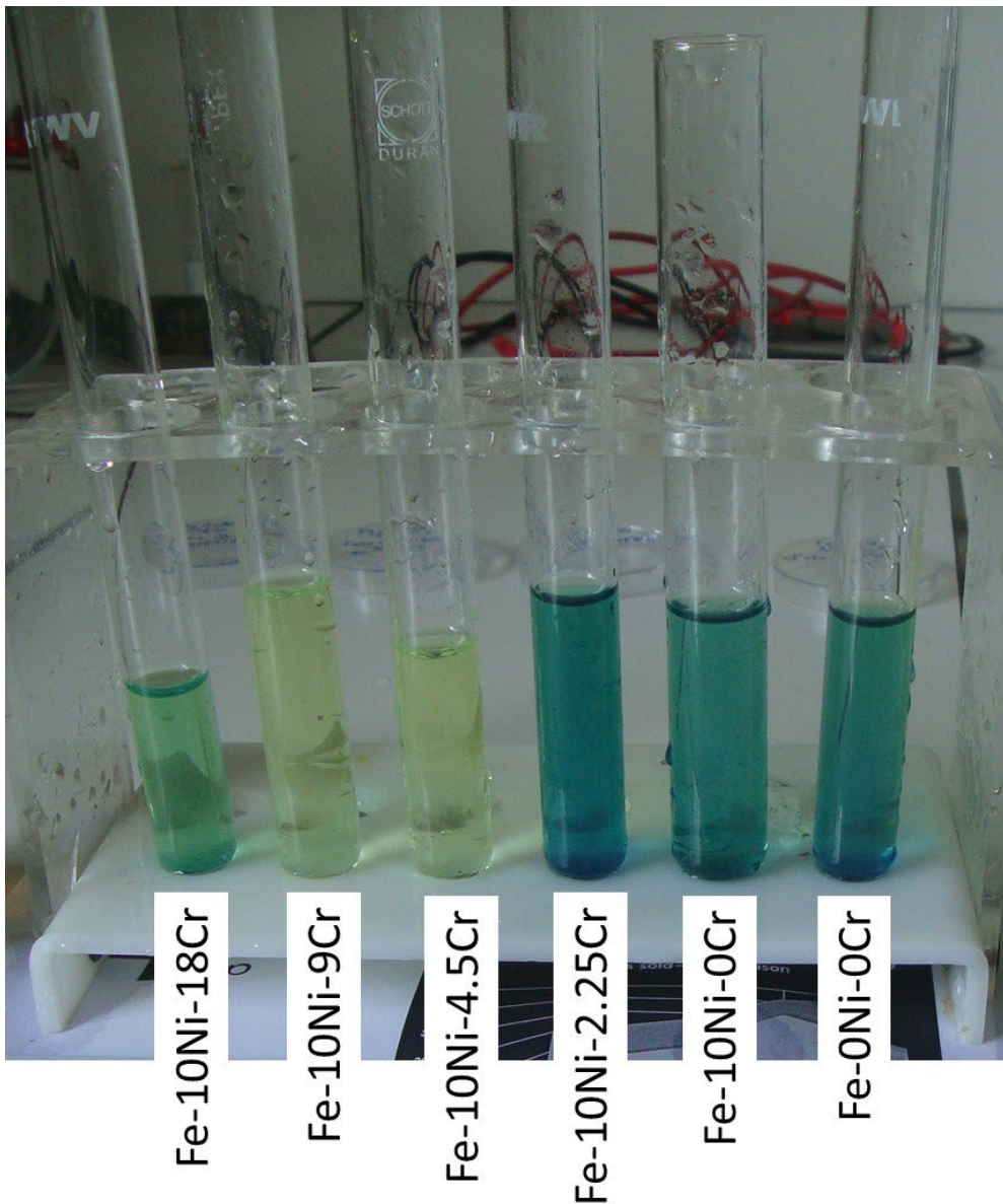
Figure 16. The series of test tubes containing the electrolyte collected in the six cells, after addition of K_3Fe(CN)_6 or K_4Fe(CN)_6 followed by acidification.
