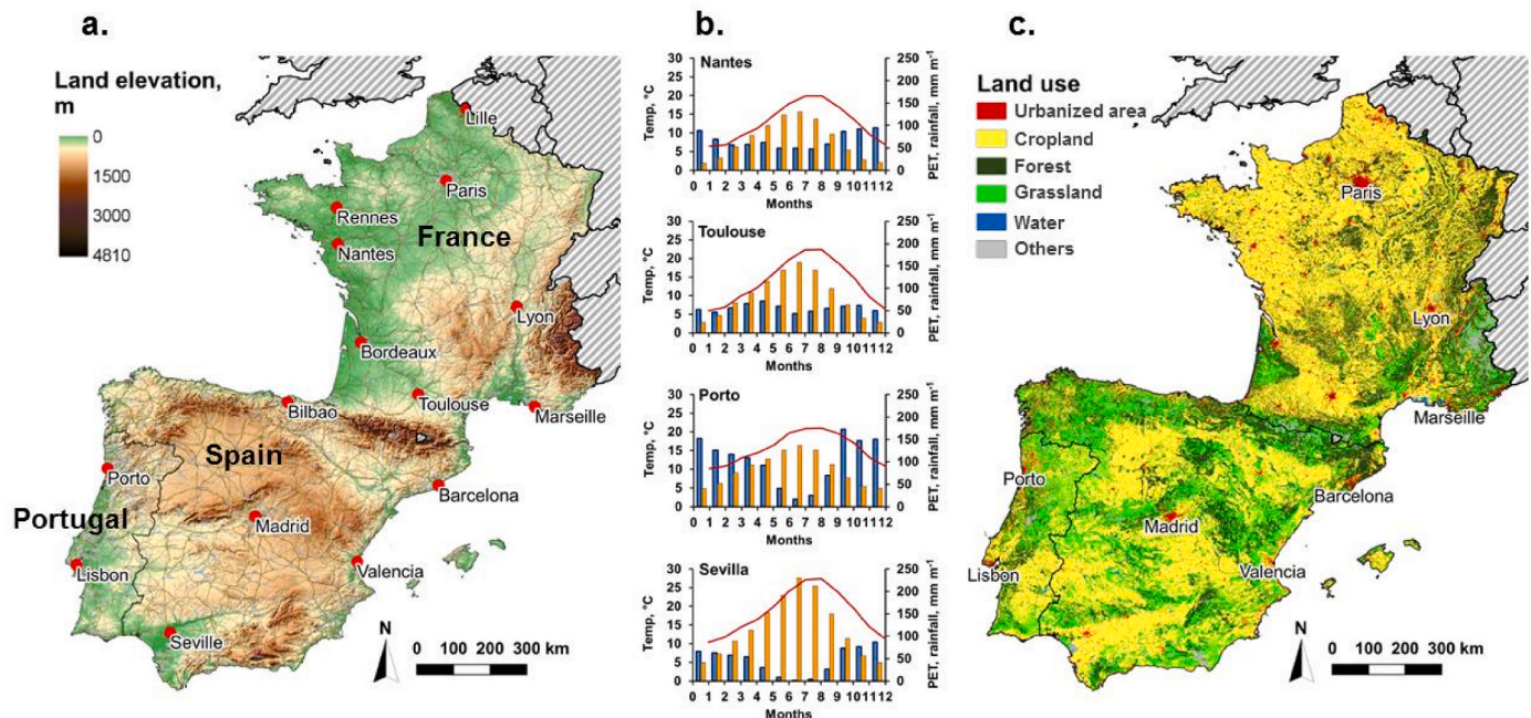
Fig. 1. a. Relief map of the study area. b. Meteorological characteristics of some cities illustrating the gradient in average monthly temperature (in °C, red line), in cumulative monthly rainfall ( \text{mm m}^{-1} , blue bar chart), and in potential evapotranspiration (PET, \text{mm m}^{-1} , orange bar chart) for the period 1990–2018. The gap in the summer period between PET and rainfall histograms represents the water deficit. c. Map of main land use (Corine Land Cover, 2018). (Cropland includes arable cropland (with temporary grassland), permanent crops, and heterogeneous areas).
