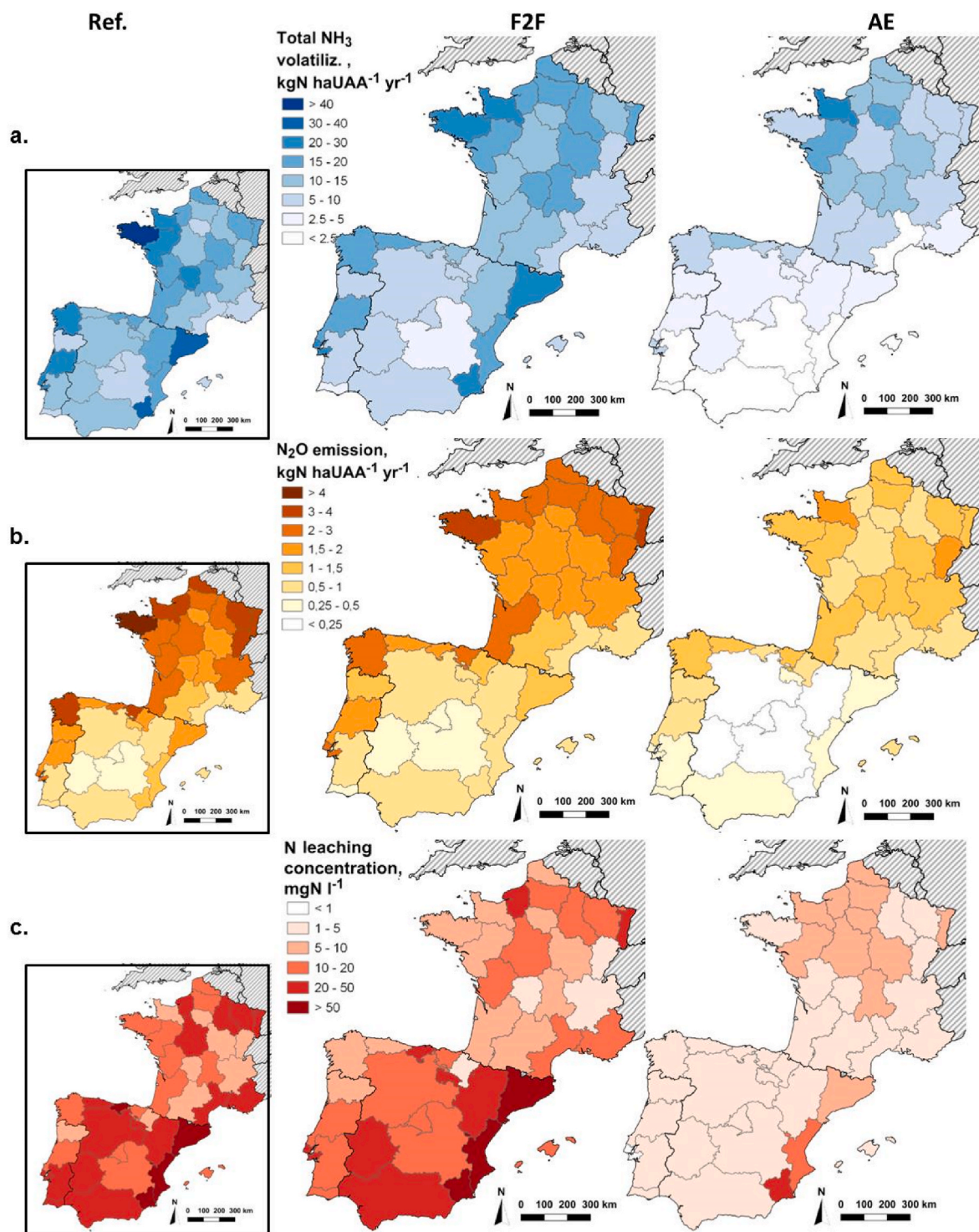
Fig. 5. Atmospheric and hydrological N losses at the regional scale of the three countries for reference (2014–2019) and the F2F and agro-ecological scenarios. a. \text{NH}_3 volatilization. b. \text{N}_2\text{O} emissions, both expressed in kg N per ha utilized agricultural area (UAA) and per year. c. N leaching concentrations, in mg N \text{L}^{-1} .
