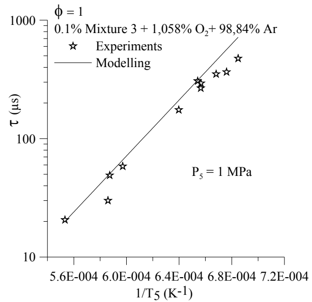
Comparison between experimental (symbols) and computed (lines) ignition delays of the Mixture 2 and 3 in a shock tube M. Yahyaoui et al., Proc. Combust. Inst. 31, 385–391 (2007)
