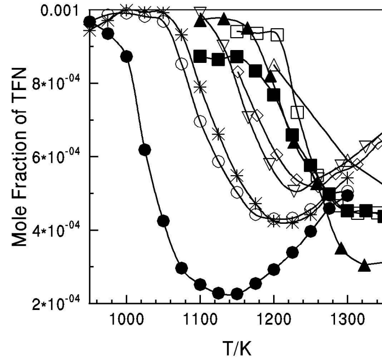
TFN (NO+HCN) vs. T for 8 reburn fuels: NG-blend ■; ethane *; ethylene ○, acetylene ●; NG △; propene □; propane ◇; n-butane △; i-butane ▲. Stoichiometric mix, 1000ppm NO, 8800 ppm C, t: 0.12-0.16s
