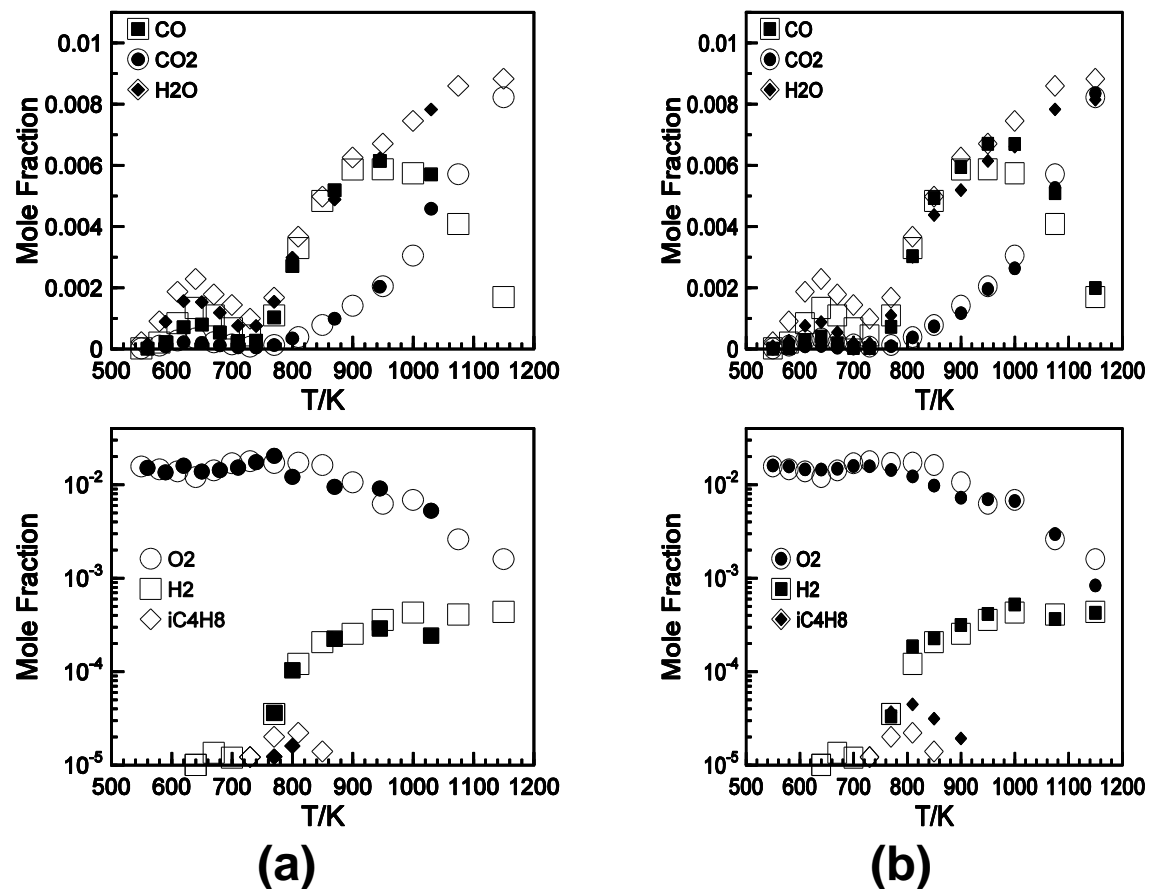
Comparison of experimental data obtained from the JSR oxidation of (a) Jet A-1 (closed symbols) and GtL (open symbols) and (b) CtL (closed symbols) and GtL jet fuel (open symbols) at \phi = 1.0 , 10 bar, and a mean residence time of 1 s. From Dagaut, P., CNF, 2014, 161(3), p. 840.
