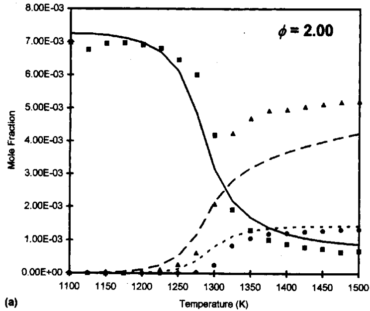
FIGURE 10 The oxidation of a \text{CH}_4/\text{C}_2\text{H}_6 (10:1) mix in a JSR at 1atm ( \tau = 0.12 s; 7272 ppm of \text{CH}_4 ; 728 ppm of \text{C}_2\text{H}_6 ; 8546 ppm of \text{O}_2 ; \phi = 2 ). Comparison between experimental data (symbols) and modeling (lines); (a) \text{CH}_4 , \blacksquare ; \text{CO} , \blacktriangle ; \text{CO}_2 , \bullet ; (b) \text{O}_2 , \square ; \text{H}_2 , \triangle ; (c) \text{C}_2\text{H}_6 , \blacksquare ; \text{C}_2\text{H}_4 , \blacktriangle ; \text{C}_2\text{H}_2 , \bullet .
