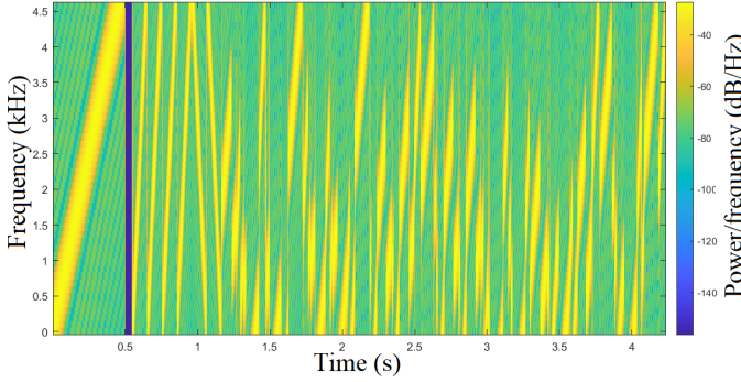
Fig. 1: Spectrogram of the transmitted signal in baseband
