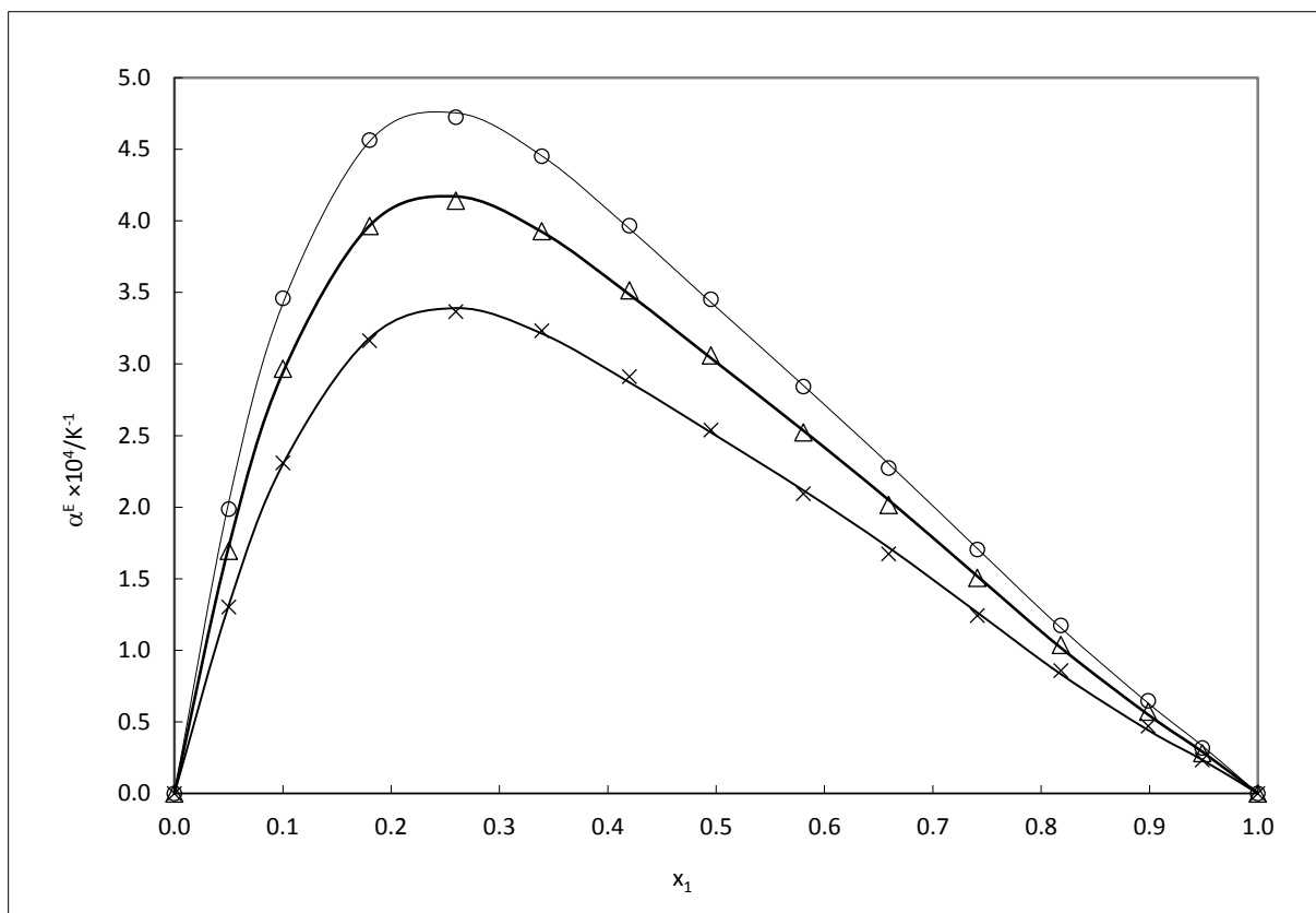
Figure 5: Excess molar expansion ( \alpha^E ) for DMI (1) + water (2) binary system as a function of DMI composition at atmospheric pressure and 3 different temperatures: (o) 293.15 K, ( \Delta ) 308.15 K, ( \times ) 328.15 K, solid line: Redlich Kister correlation.
