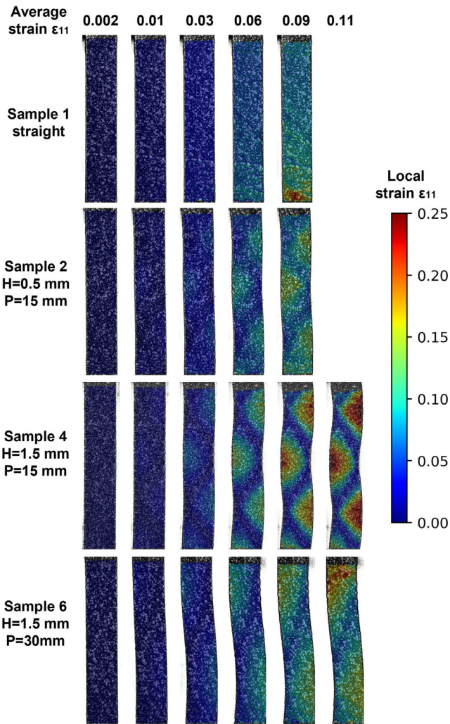
Figure 7. Strain field evolution during tensile tests on samples with different geometric patterns.
