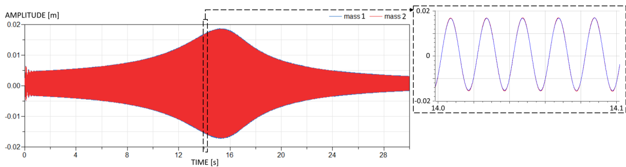
Figure 15. Mass amplitudes of the double mass–spring coupled with play ( f_r = 50 hz).
