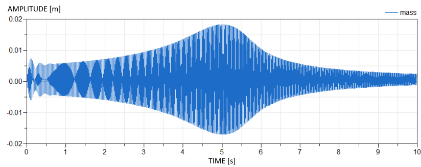
Figure 14. Mass amplitudes of the simple mass–spring coupled with play ( f_r = 50 hz).
