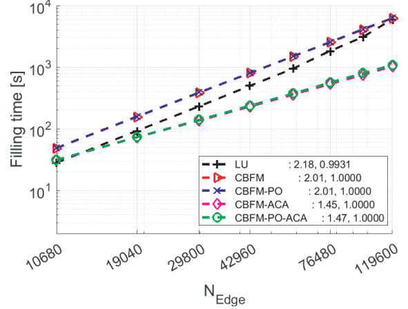
Figure 13. Filling time in seconds to calculate the whole impedance matrix (for LU) and the sub-matrices of CBFM. The EFIE is applied.
