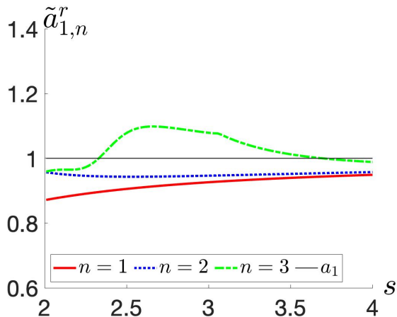
(a) Exact data. Regularization.
