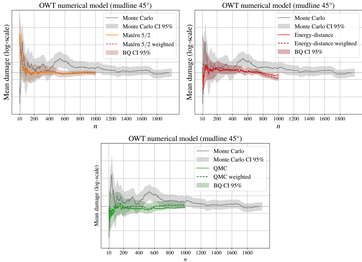
Figure 16: Mean estimation convergence (at the mudline, azimuth \theta = 45 deg.) on the Teesside case
