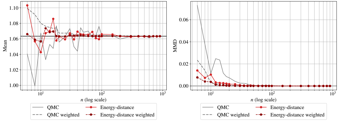
Figure 12: Analytical benchmark results on the toy-case #1
