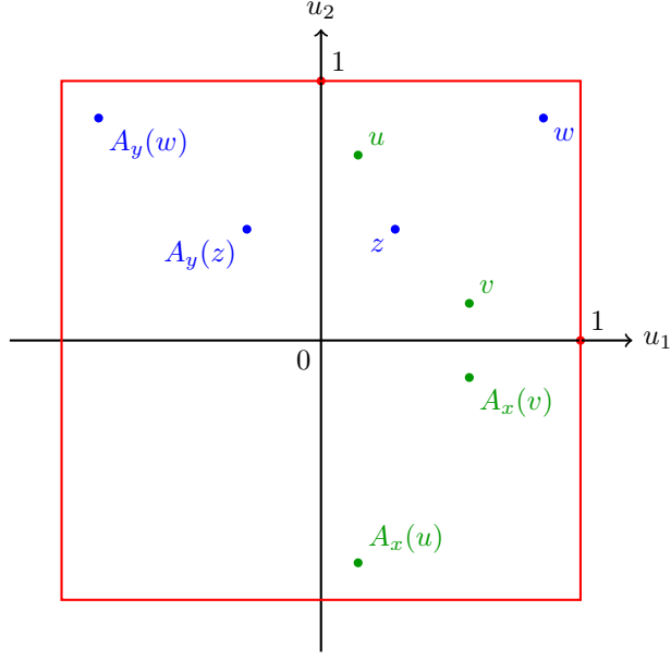
Figure 1: Mirror-type transformation with d = 2 , for x = (1/3, 3/4) , and for y = (2/3, 1/5) .
