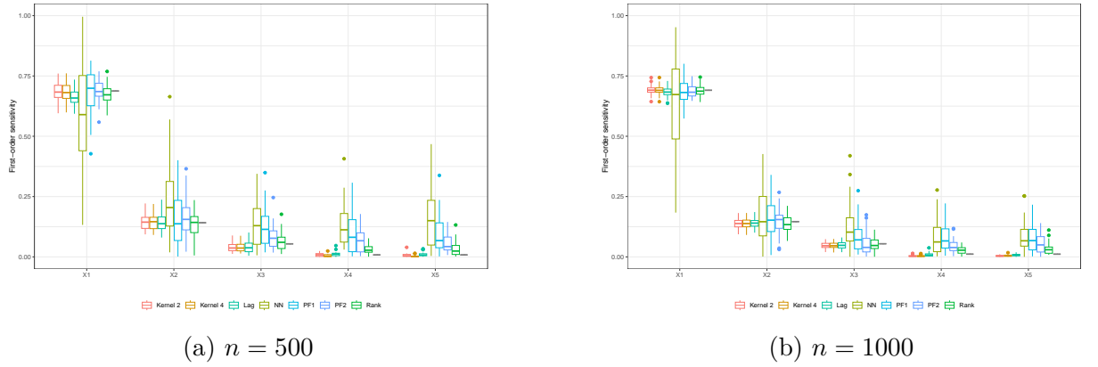
Figure 3: Estimators for first-order indices of the Bratley function with n = 500 (left) and n = 1000 (right). The reference value is represented with a gray line.
