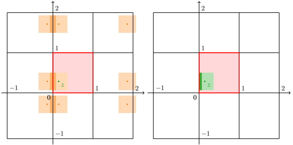
Figure 2: Mirror-image transformation with d = 2 in red. In the left-hand side of the figure, a data-point in [0, 1]^d (in green) and its 8 mirror-images (in orange). A kernel is fitted over all points of the augmented dataset (orange areas). The darker orange regions correspond to the regions where several kernels overlap. In the right-hand side of the figure, the data-point (in green) and the restriction to [0, 1]^d of the augmented dataset (in green).
