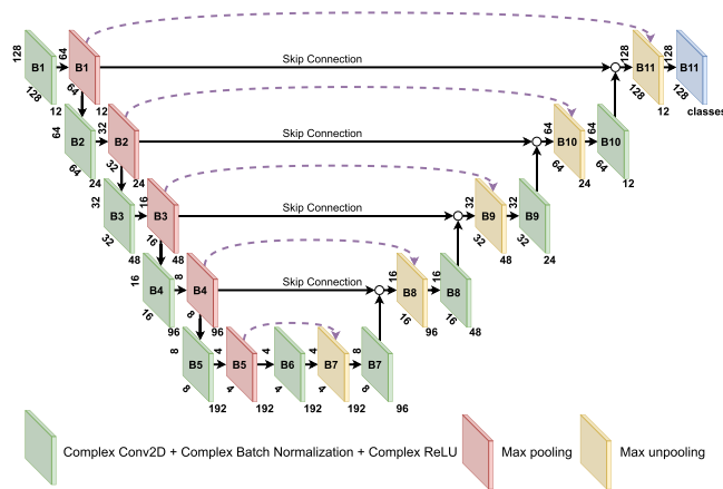
FIGURE 1. Complex-Valued Fully Convolutional Neural Network (CV-FCNN) diagram.
