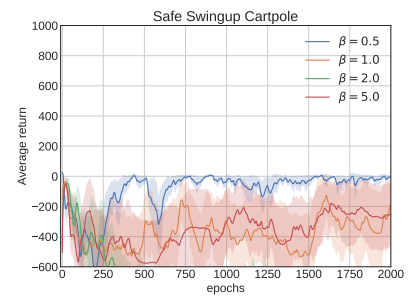
(c) Cartpole Swingup
