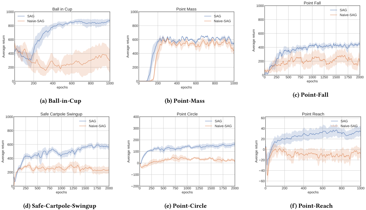
Figure 7: Comparison between the Empirical Bellman Operators used on SAG on all environments.
