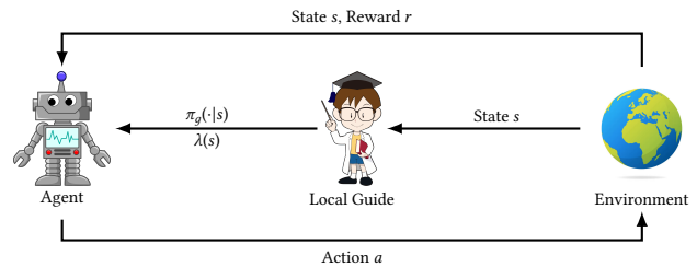
Figure 1: Reinforcement Learning with Local Guides
