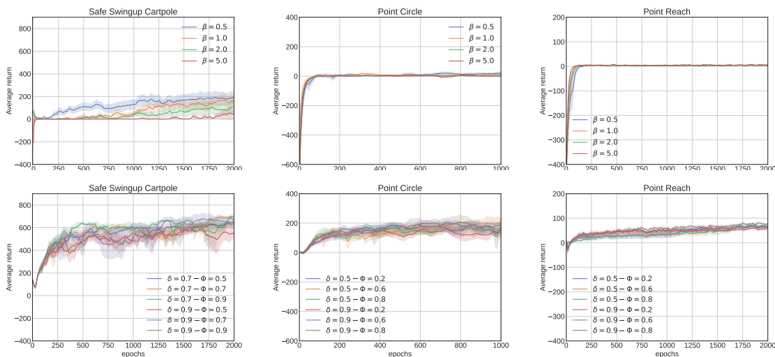
Figure 5: Hyper-parameter analysis of PIG (top) and PAG (bottom) on environments with repulsive policies.
