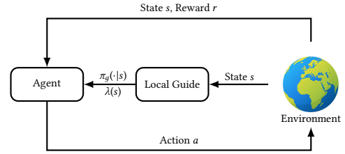
Figure 1: Reinforcement Learning with Local Guides
