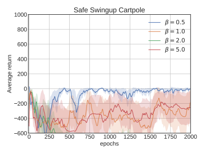
(c) Cartpole Swingup
